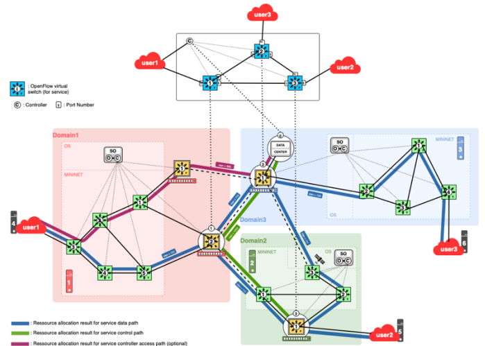
FIGURE 7 PROVISIONED RESOURCES
