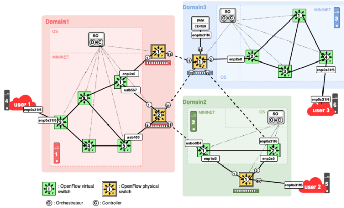
FIGURE 4 NETWORK SET-UP
