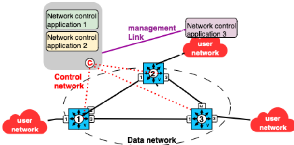
FIGURE 2. SERVICE COMPONENTS
