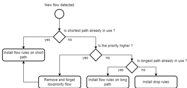
Figure 9: Demonstration dedicated control application working flow
