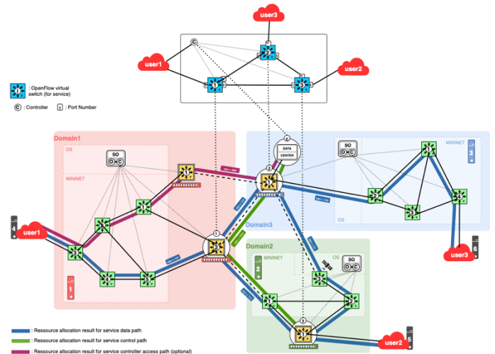
FIGURE 7 PROVISIONED RESOURCES
