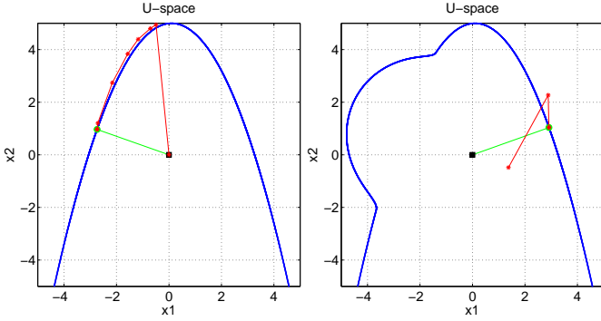
Figure 1. Parabolic limit-state function: FORM with search for multiple design points.
