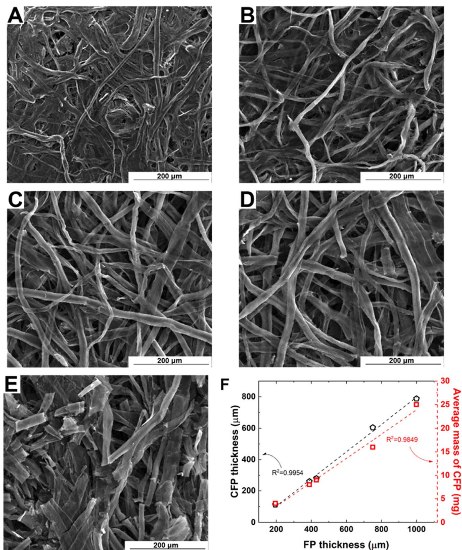
Fig. 2 Morphology characterization of CFP electrodes: SEM micrographs (A) CFP 195 ; (B) CFP 390 ; (C) CFP 430 ; (D) CFP 700 ; (E) CFP 1000 ; and (F) correlation of precursor (FP) thickness and CFP electrode thickness and mass.
