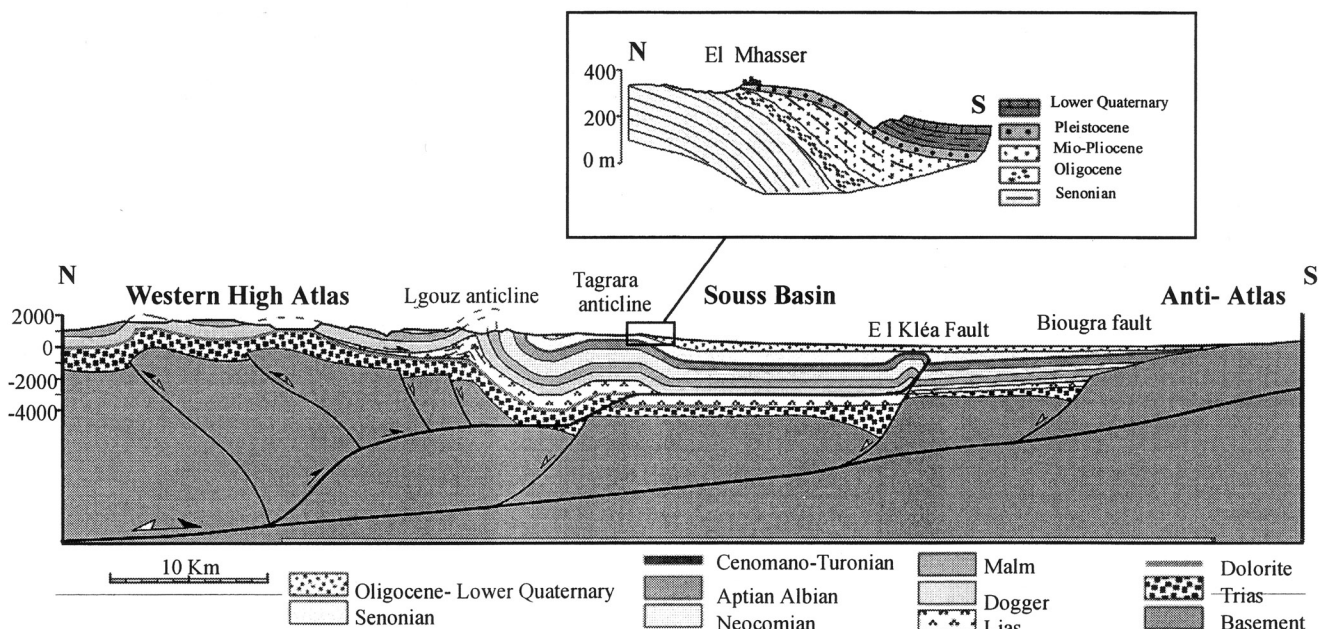
Figure 6. Generalized cross-section through the Souss basin and the Western High Atlas (modified and completed from Outtani [1996] and Mustaphi [1997]; sources of data are field work and Office National de Recherche et Exploration Pétrolières (ONAREP) seismic profiles). See explanations in the text and location in Figure 5. Insert shows the geometry of Tertiary and Quaternary series along the front of the Tagrara anticline (modified from Ambroggi [1963]).
