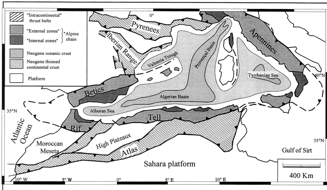
Figure 1. Schematic map of the western Mediterranean region showing the main orogens and extensional basins (modified from Dogliani et al. [1999], s.l., sensu lato ).
