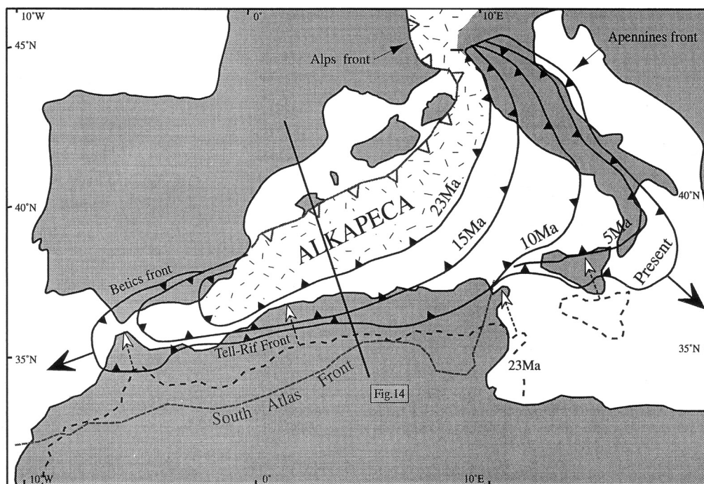
Figure 13. Schematic map illustrating the successive geometry of the Tell-Rif-Apennine subduction starting in the western Mediterranean during Oligocene (strongly modified for the western region from Dogliani et al. [1999]). See discussion in the text. ALKAPECA: Alboran, Kabylies, Peloritian, and Calabria.
