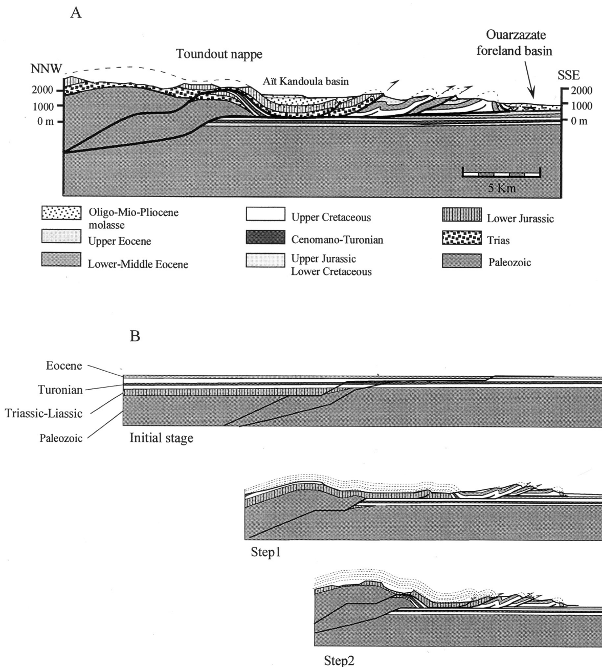
Figure 9. (a) Cross section through the southern part of the Central High Atlas (strongly modified from Errarhaoui [1997]; source of data are field mapping and ONAREP seismic profiles). See explanations in the text and location in Figure 8. (b) Schematic kinematic evolution of the cross-section in Figure 9a. See explanations in the text.
