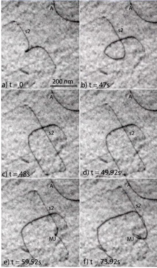
Figure 9: Glide motion of a screw dislocation s2 of variable length at 523 K (same zone as in Fig. 8). See corresponding video as Supplementary material.
