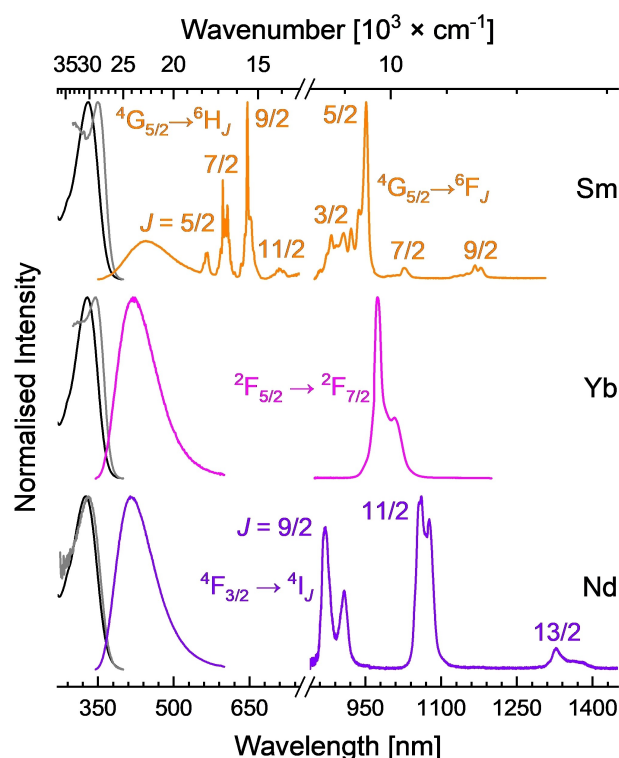
Figure 5. Normalised absorption (black), excitation (grey, \lambda_{\text{exc}}=645 nm for Sm, 976 nm for Yb and 1059 nm for Nd) and emission ( \lambda_{\text{em}}=331 nm, Sm; orange; Yb: magenta, Nd: violet) spectra of LnL 3 complexes (Ln = Sm, Yb, Nd, [ LnL 3 ] \approx 1 –2 \mu M) in MeOH.
