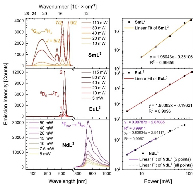
Figure 6. Left: 2 P (Ln = Sm, Eu; in MeOH) and 1 P (Ln = Nd; in \text{CH}_2\text{Cl}_2 ) emission spectra of \text{LnL}^3 complexes. Right: plots of the Sm, Eu and Nd emission intensities at 640, 620 and 871 nm versus incident average laser power for Sm , Eu and NdL 3 on a log/log scale. The fits of the experimental data (shown in black scatter) are shown as coloured lines, fitted model function, the obtained parameters and standard deviations are reported in insets. The scales on the right plots represent emission intensity [counts] as on the left emission spectra, \lambda_{\text{exc}} = 700 (Sm, Nd) or 710 (Eu) nm, [\text{SmL}^3] = [\text{NdL}^3] = 10 \mu\text{M} , [\text{EuL}^3] = 3.2 \mu\text{M} .
