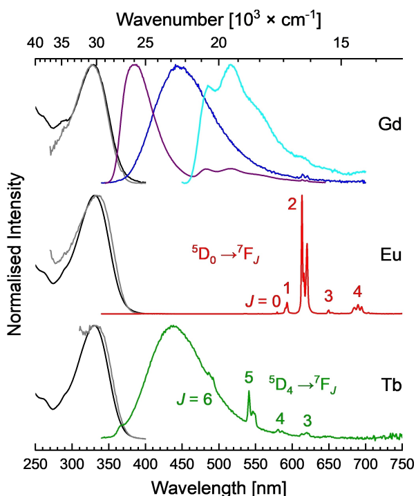
Figure 3. Normalised absorption (black), excitation (grey, \lambda_{\text{em}} = 415 nm for Gd, 613 nm for Eu and 541 nm for Tb) and emission spectra of \text{LnL}^3 complexes ( \text{Ln} = \text{Eu}, \text{Gd}, \text{Tb} , [\text{LnL}^3] \approx 1\text{--}2\ \mu\text{M} ) in MeOH in aerated conditions ( \lambda_{\text{exc}} = 328 or 330 nm, Gd: blue at 293 K, purple at 77 K, cyan at 77 K after 0.05 ms delay; Eu: red; Tb: green). \text{GdL}^3 spectra at 77 K were measured in EtOH:MeOH (4:1).
