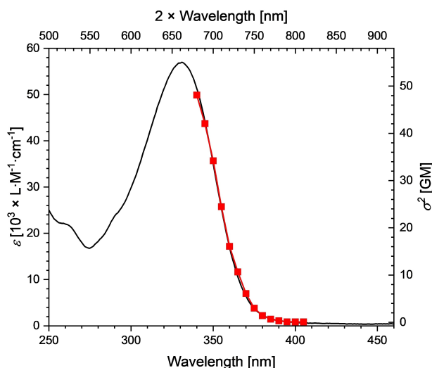
Figure 7. Two-photon excitation (red line and scatter) and one-photon absorption (black line) spectra of EuL 3 in MeOH, [EuL 3 ] = 3.2 \mu\text{M} . The bottom and top scales correspond to the wavelength of one- and two-photon spectra, respectively.
