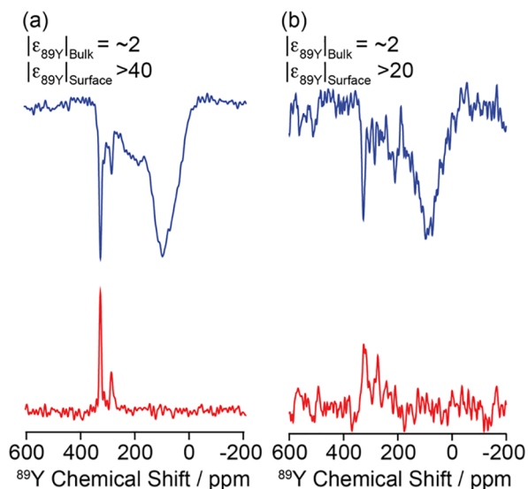
Figure 4. Direct ^{89}\text{Y} DNP-enhanced MAS NMR spectra of (a) 0.1% \text{Gd}_2\text{O}_3 -added \text{Y}_2\text{O}_3 and (b) \text{Y}_2\text{O}_3 , recorded with \mu_w on (blue) and \mu_w off (red). All NMR data were recorded with recycle delays of 120 s and trityl as a polarizing agent at the negative maximum of the field profile ( B_0 = 9.3975 T).
