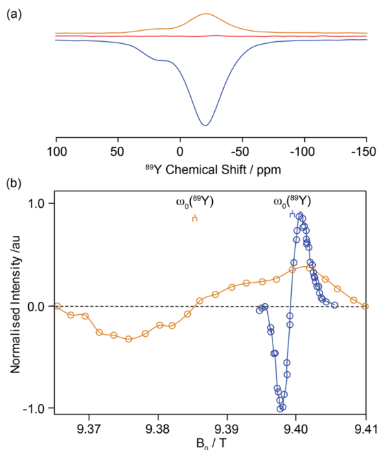
Figure 3. 89 Y MAS NMR spectra and MAS DNP field profiles for Y(NO 3 ) 3 in solution. (a) 89 Y MAS DNP NMR spectra of Y(NO 3 ) 3 in a solution of glycerol- d 8 /D 2 O/H 2 O in a 6:3:1 ratio (v/v) with \mu_w on for trityl (blue) and AMUPol (orange) and \mu_w off (red). Only the isotropic resonances are shown. (b) 89 Y MAS DNP field profiles for binitroxide radical AMUPol 28 (orange) and trityl 25 (blue). The intensities are normalized to the maximum signal obtained. \omega_0(^{89Y}) is shown centered to the isotropic resonance of the corresponding radicals.
