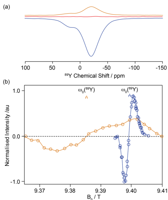
Figure 3. ^{89Y} MAS NMR spectra and MAS DNP field profiles for Y(NO_3)_3 in solution. (a) ^{89Y} MAS DNP NMR spectra of Y(NO_3)_3 in a solution of glycerol- d_8 /D 2 O/H 2 O in a 6:3:1 ratio (v/v) with \mu_w on for trityl (blue) and AMUPol (orange) and \mu_w off (red). Only the isotropic resonances are shown. (b) ^{89Y} MAS DNP field profiles for binitroxide radical AMUPol 28 (orange) and trityl 25 (blue). The intensities are normalized to the maximum signal obtained. \omega_0(^{89Y}) is shown centered to the isotropic resonance of the corresponding radicals.
