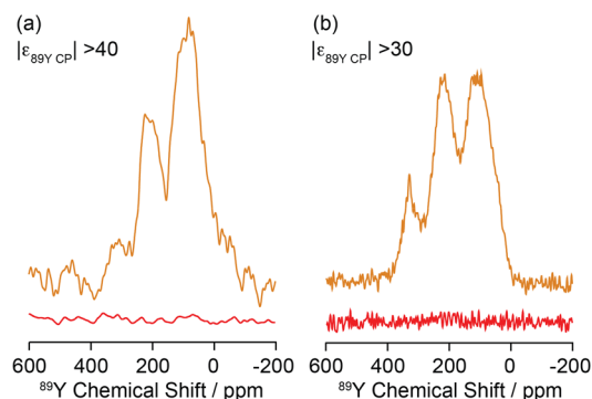
Figure 6. DNP-enhanced \{^1\text{H}\}\text{Y} CP MAS NMR spectra of yttrium oxides. (a) 0.1% \text{Gd}_2\text{O}_3 -added \text{Y}_2\text{O}_3 with a CP contact time of 8 ms and (b) \text{Y}_2\text{O}_3 with a contact time of 20 ms, recorded with \mu\text{w} on (orange) and \mu\text{w} off (red). Note that fewer scans were collected in (b). All \{^1\text{H}\}\text{Y} CP MAS NMR spectra were recorded with AMUPol at the positive maximum of the ^1\text{H} CE ( B_0 = 9.395 T).
