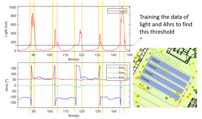
Fig. 6. Light intensity determined CRPs in IOT2US system.
