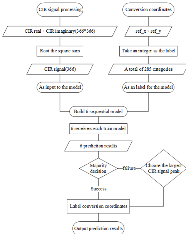
Fig. 41. Flow chart of the system proposed by YAI team for CIR-based positioning.
