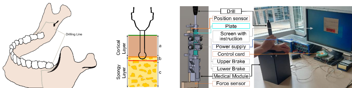
Figure 1: Left: jawbone drilling along the Epker line. Middle: schematic representation of the drilling task with the different layers: a) cortical sensation, b) transitory sensation, c) spongy sensation. Right: drilling haptic simulator and components.
