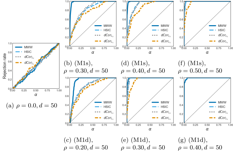
Figure 7: Plots of the rejection rate under \mathcal{H}_0 (a) and \mathcal{H}_1 (b-g) against the significance level \alpha \in (0, 1) for (M1s) top row, and (M1d) bottom row, with \phi(u) = u ( \text{rForest}_{MWW} ), \rho = 0.0 (a) \rho \in (0.20, 0.50) (b-g). The parameters are fixed to N = 500 , d = 50 , K_p = 10 , K_0 = 200 , B = 100 for all experiments.
