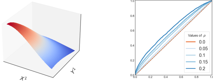
Figure 1: Left: Joint Gaussian density for \rho = 0.20 of (X^1, Y^1) . Right: Plots of the optimal ROC curves for two Gaussian vectors with linear correlation \rho \in \{0.0, 0.05, 0.10, 0.15, 0.20\} and q = l = 5 .
