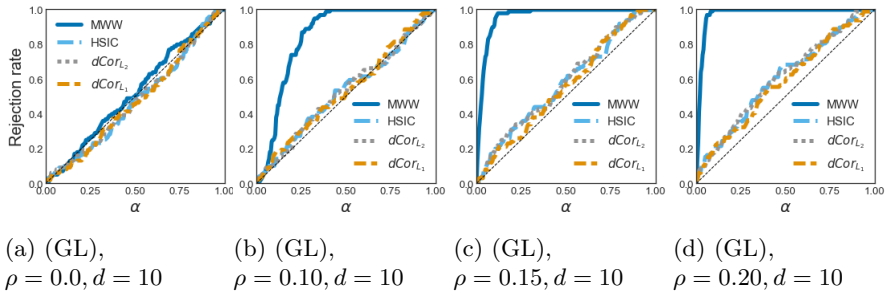
Figure 4: Plots of the rejection rate under \mathcal{H}_0 (a) and \mathcal{H}_1 (b-d) against the significance level \alpha \in (0, 1) for (GL) with \phi(u) = u ( rForest MWW ), \rho = 0.0 (a) \rho = 0.10 (b), \rho = 0.15 (c), \rho = 0.20 (d). The parameters are fixed to N = 1000 , d = 10 , K_p = 10 , K_0 = 200 , B = 100 for all experiments.
