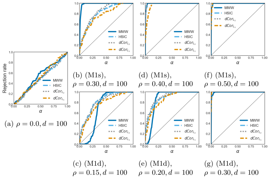
Figure 8: Plots of the rejection rate under \mathcal{H}_0 (a) and \mathcal{H}_1 (b-g) against the significance level \alpha \in (0, 1) for (M1s) top row, and (M1d) bottom row, with \phi(u) = u ( \text{rForest}_{MWW} ), \rho = 0.0 (a) \rho \in (0.15, 0.50) (b-g). The parameters are fixed to N = 500, d = 100, K_p = 10, K_0 = 200, B = 100 for all experiments.
