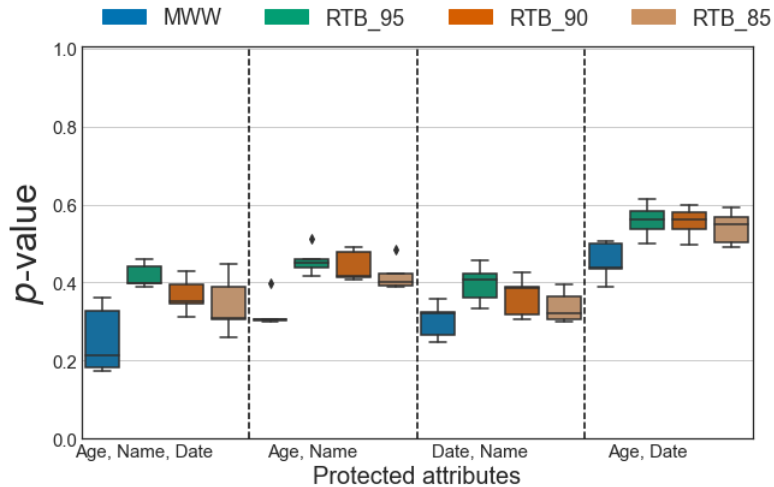
Figure 5: Boxplots of the p -values for different sets of protected attributes. The experimental parameters are fixed to N = 10^3 , K_p = 10 , q = 1 , l \in \{2, 3\} , 5-fold cross-validation, 31 features, based on the open-source dataset available [33].
