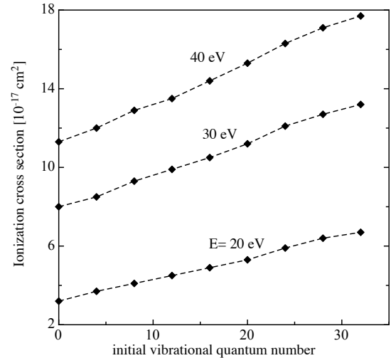
Fig. 9. Total ionization cross section for the process O 2 ( X^3\Sigma_g^-, v ) + e \rightarrow O 2 + ( X^2\Pi_g, a^4\Pi_u, A^2\Pi_u, b^4\Sigma_g^- ) as a function of the initial vibrational quantum number for different collision energies, calculated by Kosarim et al [236].
