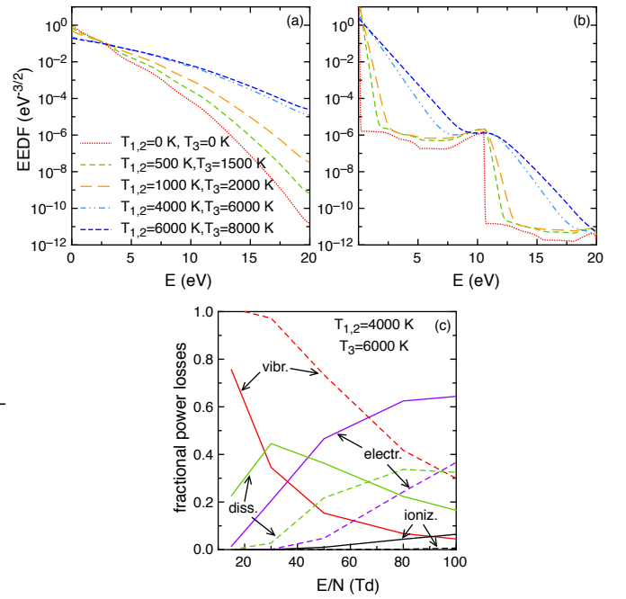
Fig. 15. CO 2 EEDF calculated with the parametric solution of the electron Boltzmann equation in (a) discharge (E/N=30 Td) and (b) post-discharge (E/N=0 Td) conditions at different T_{1,2} and T_3 temperatures [265]. (c) Fractional power losses as a function of E/N at T_{1,2}=4000 \text{ K} and T_3=6000 \text{ K} (full lines) and in the cold gas approximation ( T_{1,2}=T_3=0 \text{ K} ) (dashed lines) [266].
