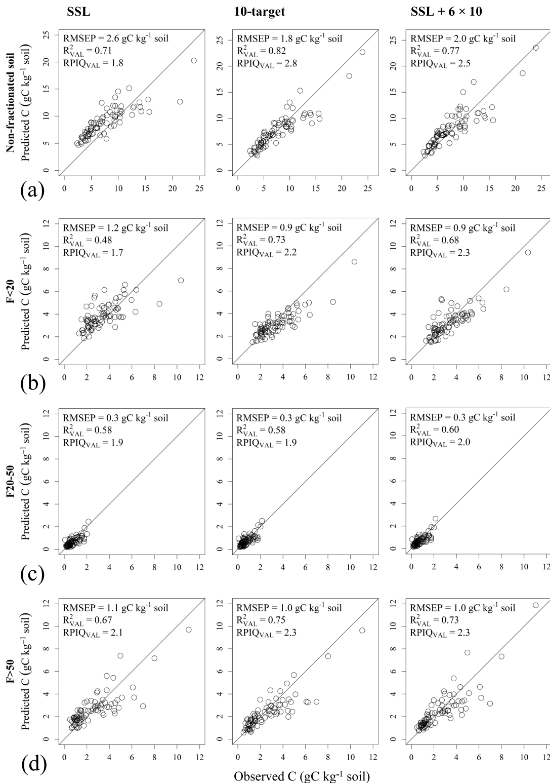
Fig. 4. Observed vs. predicted C amounts (gC kg -1 soil) in (a) the non-fractionated soil, and the particle size fractions (b) 0–20 μm (F<20), (c) 20–50 μm (F20-50), and (d) 50–2000 μm (F>50), for the validation set, using three calibration datasets: (i) the spectral library alone (SSL), (ii) the 10-target alone, and (iii) SSL with 10 spiking samples extra-weighted six times (SSL+6×10). In each case, the model shown was obtained with the spectral pretreatment (i.e. raw or pretreated) and the PLSR method that minimized RMSEP (global PLSR for the non-fractionated soil, local PLSR for the fractions). The line represents y = x .
