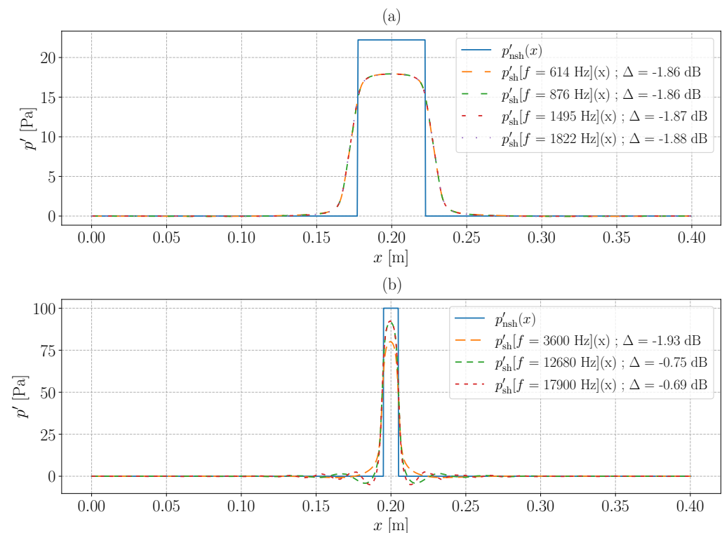
Figure A1. Acoustic pressure p' distribution along the laser beam axis x at t_{\max} . L_{\text{AO}} = 2.6 \times 10^{-9} m, n_0 = 1.00026 , \beta = 2.6 \times 10^{-9} Pa ^{-1} and L_0 = 0.4 m. (a) Waveguide No. 1. (b) Waveguide No. 2. Refer to Table 1 for waveguides parameters.
