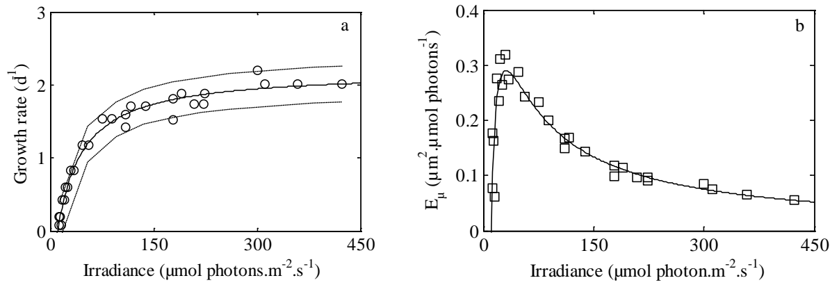
Figure 2: a) Growth rate as a function of irradiance: experimental data (open circles) were fitted with equation 1 (solid line; r^2 = 0.97 ). The lower and upper dotted lines represent the 95 % confidence boundaries. b) Irradiance efficiency for growth rate ( E_{\mu} ) on irradiance for optically clear cultures.
