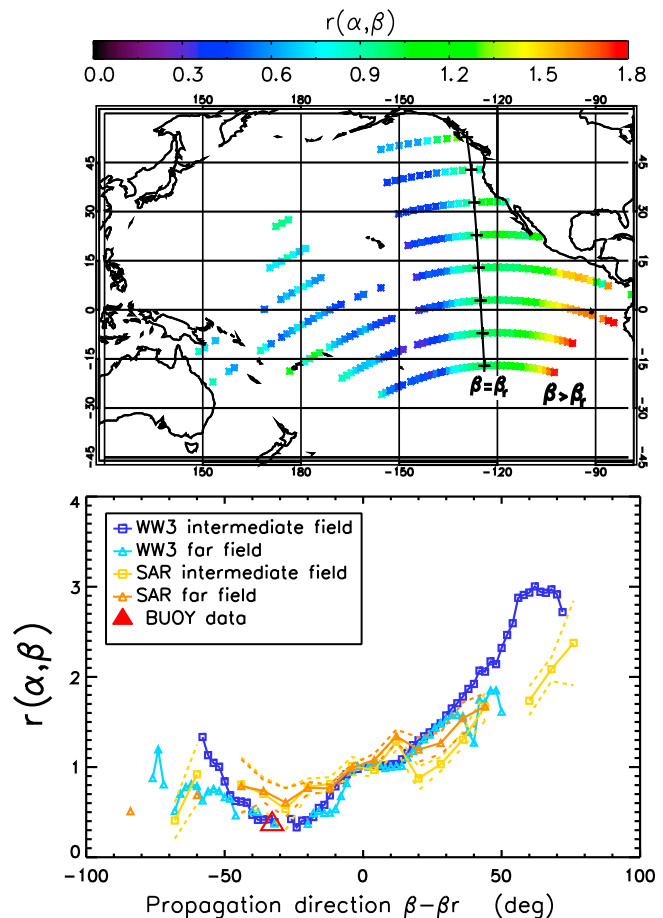
Figure 7. Same as Figure 6 but for the storm which occurred on 9 August 2004 at 0000 UTC, located at 120°W, 57°S.
