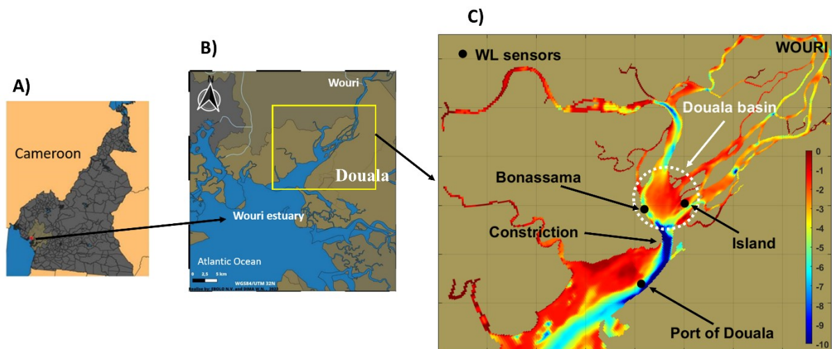
19 Fig. 1. Geographical location of the Wouri estuary. A: Map of Cameroon. B: Map of the Wouri 20 estuary. C: Bathymetry of the upper part of the estuary where the Douala basin is located. The black 21 dots correspond to the positions of the water-level sensors used in this study.
