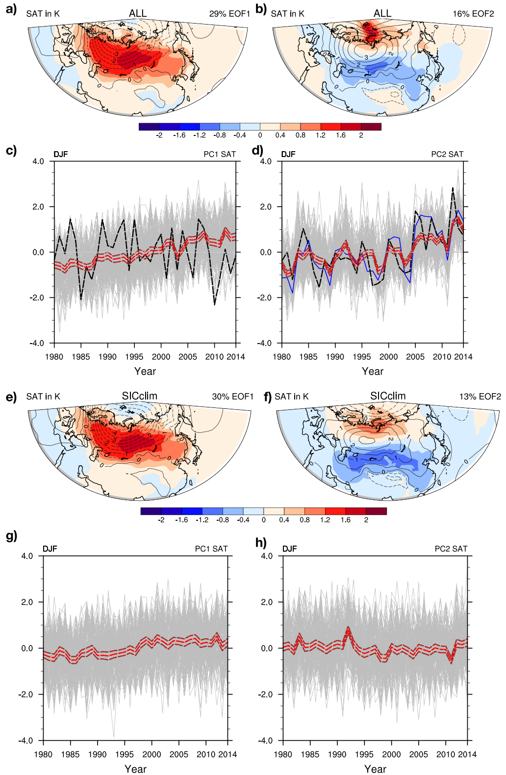
Figure 3. The multi-model mean (a) EOF1 and (b) EOF2 patterns in the winter (DJF) SAT (in K) over Eurasia ( 20^{\circ} N– 90^{\circ} N, 0^{\circ} – 180^{\circ} E) in ALL with daily year-to-year varying observed SST and SIC conditions for the period of 1980–2014. The black contours are the multi-model mean SLP (in hPa) fields associated with the EOFs, derived by regression of the SLP on the respective normalised PC time series for each model. (c) The normalised PC1 time series in grey for the 145 ensemble members of the ALL . The black line is the same but from ERA5 data for 1980–2014. The red line is the ensemble mean of the PC1 time series, and the brown lines are the 95% confidence intervals of the ensemble mean. (d) As in (c) but for the PC2, i.e. WACE mode. The other blue curve is the normalised sign reversed time series of the observed area averaged winter SIC anomalies in BKS from HadSST1 ( 65^{\circ} N– 85^{\circ} N, 20^{\circ} E– 90^{\circ} E, blue box in figure 1(a)). (e)–(h) are the same as (a)–(d) but for the SICclim experiment with daily climatological Arctic SIC forcing instead of year-to-year varying SIC. Top right corners of (a), (b), (e), (f) mention the multi-model mean of the percentages of the total variance explained by the respective EOFs.
