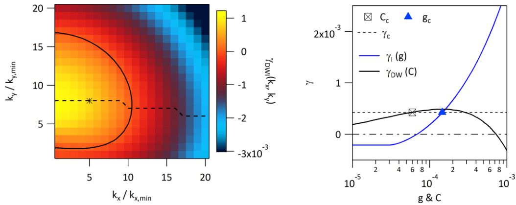
Figure 1: Left hand side, instability growth rate \gamma_{Dwl}(k_x, k_y) with mixed Drift Wave + Interchange conditions, g = 1.5 \cdot 10^{-4} and C = 6.0 \cdot 10^{-5} versus the wave numbers k_x and k_y . The steps in k_x and k_y , k_{x,min} and k_{y,min} , are \pi\rho_* with 1/\rho_* = 256 . The black contour is plotted for \gamma_{Dwl} = 0 . The dashed black line is the line of k_y values at the maximum of the growth rate \gamma_{Dwl} at given k_x and the star symbol locates the value for k_x = 5k_{x,min} . Right hand side, maximum growth rate for k_x \geq 5k_{x,min} and all values of k_y , blue curve maximum of \gamma_l(g) versus g for Interchange without drift waves, black curve maximum of \gamma_{DW}(C) versus C for Drift Waves without interchange. For g_c = 1.5 \cdot 10^{-4} and C_c = 6.0 \cdot 10^{-5} , open black square marker and closed blue triangle respectively, the growth rate values are equal \gamma_l(g_c) = \gamma_{DW}(C_c) = \gamma_c .
