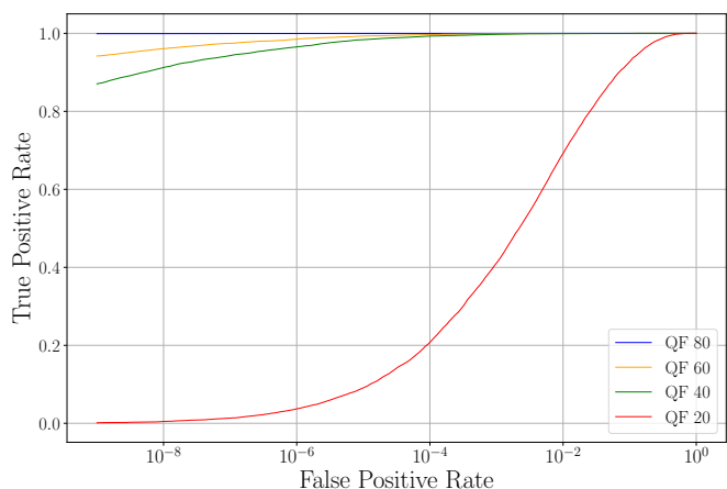
Fig. 5. True positive rate for watermarked images of size 512 \times 512 compressed with different JPEG quality factors as a function of Gaussian FP rate.
