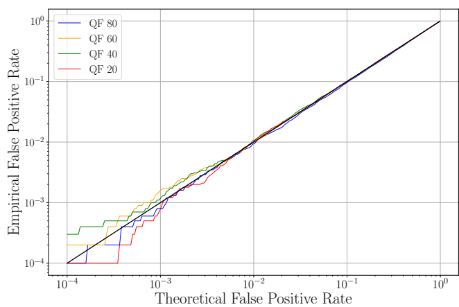
Fig. 4. False positive rate: theoretical vs empirical check for 512 \times 512 images JPEG compressed with different quality factors.
