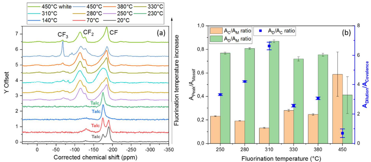
Figure 3: (a) Normalised ^{19}\text{F} NMR spectra of FCF samples, (b) evolution of the ^{19}\text{F} NMR CF peak relative areas depending on the fluorination temperature [print with colour]
