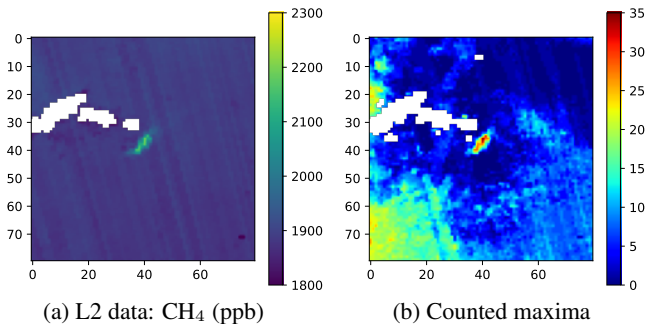
Fig. 1: Figure (a) shows the concentration of methane in parts per billion (ppb) given by the L2 methane product from Sentinel-5P. We see a methane plume in green. Pixels in white are discarded pixels (cloudy for example). Figure (b) gives the number of counted maxima for each pixel in the original image computed with the proposed method.
