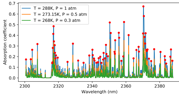
Fig. 2: Comparison of methane absorption spectra under several pressure/temperature conditions. Red dots highlight the 70 maxima we use for detecting the plumes.
