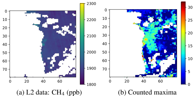
Fig. 3: In the center of (a) we see a methane plume. We detect this plume in our result (b). But we also find two other plumes below the first one that cannot be seen in the L2 product. Note that less pixels are discarded in our image than in the L2 product.
