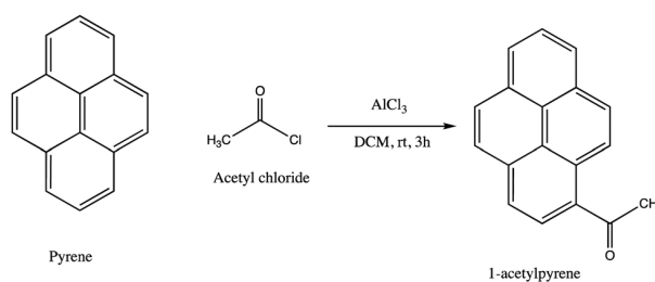
Scheme 2 Friedel-Crafts acylation between pyrene and acetyl chloride. 16
