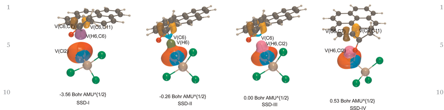
Fig. 9 ELF basin isosurfaces ( \eta = 0.72 ) of each of the SSDs found along the reaction path- b (TS2- b ).
