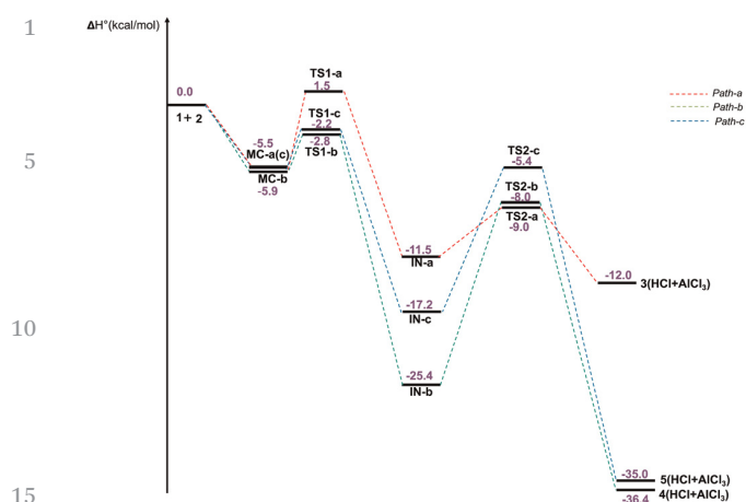
Fig. 3 Relative enthalpy energy profile along the three competitive paths (a, b, and c), in kcal mol -1 , for the stationary points involved in the Friedel–Crafts reaction of pyrene ( 1 ), evaluated at the \omega B97X-D/6-311G(d,p) level and in DCM.
