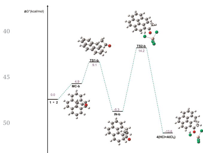
Fig. 4 Relative Gibbs free energy profile (path-b), in kcal mol -1 , for the stationary points involved in the Friedel–Crafts reaction of pyrene ( 1 ), evaluated at the \omega B97X-D/6-311G(d,p) level and in DCM.
