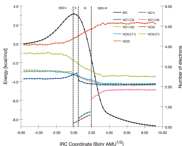
Fig. 6 Population evolution (in electrons) of selected basins along the IRC path corresponding to path- b (TS1-b).
