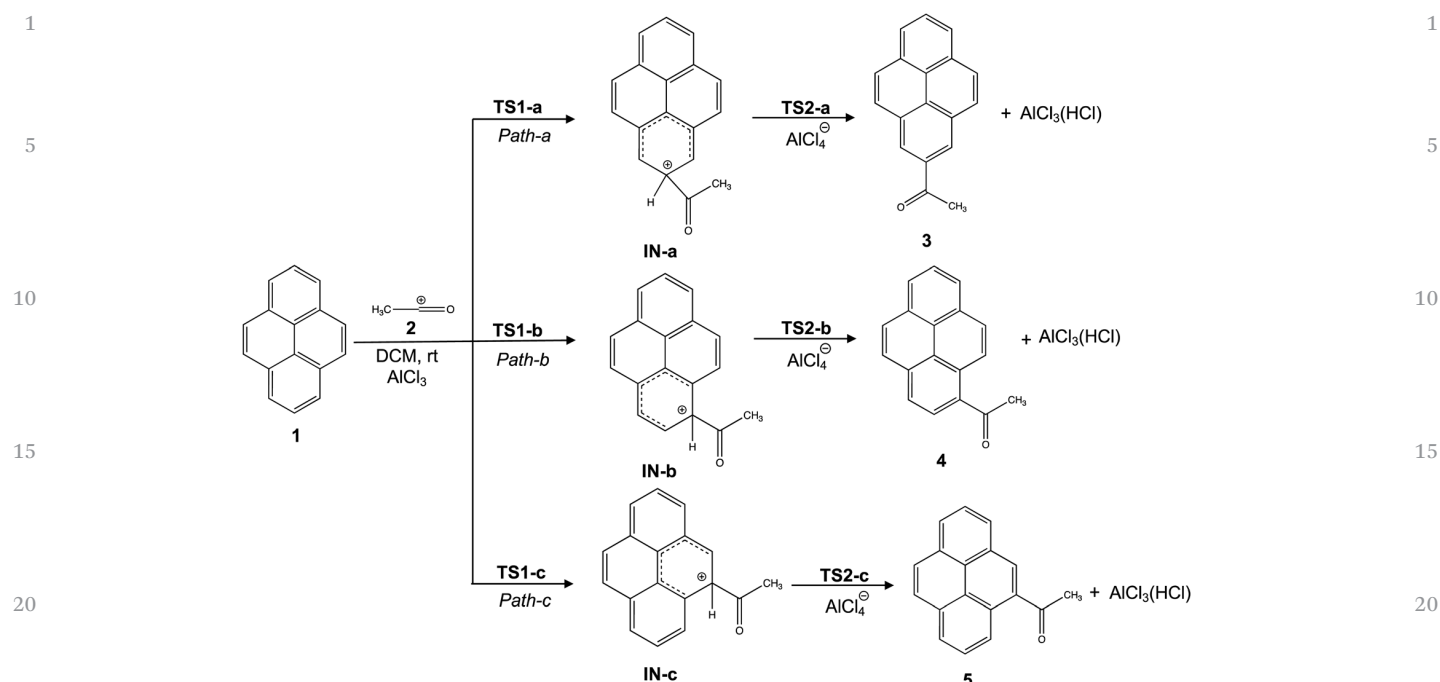
Scheme 3 Competitive reaction pathways associated with the acylation of pyrene (1) with the methylacylium ion (2).
