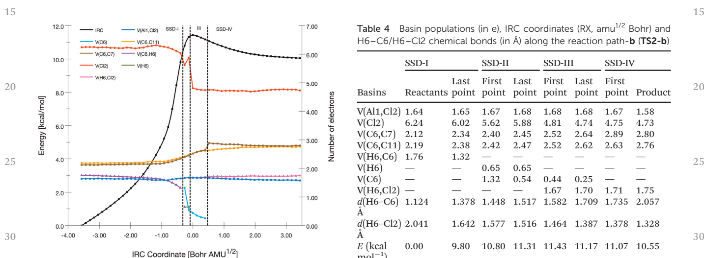
Fig. 8 Population evolution (in electrons) of selected basins along the IRC path corresponding to path- b (TS2-b).
