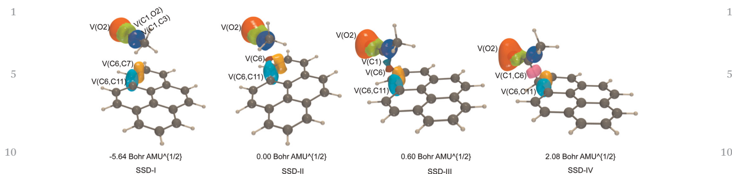
Fig. 7 ELF basin isosurfaces ( \eta = 0.72 ) of each of the SSDs found along reaction path- b (TS1-b).
