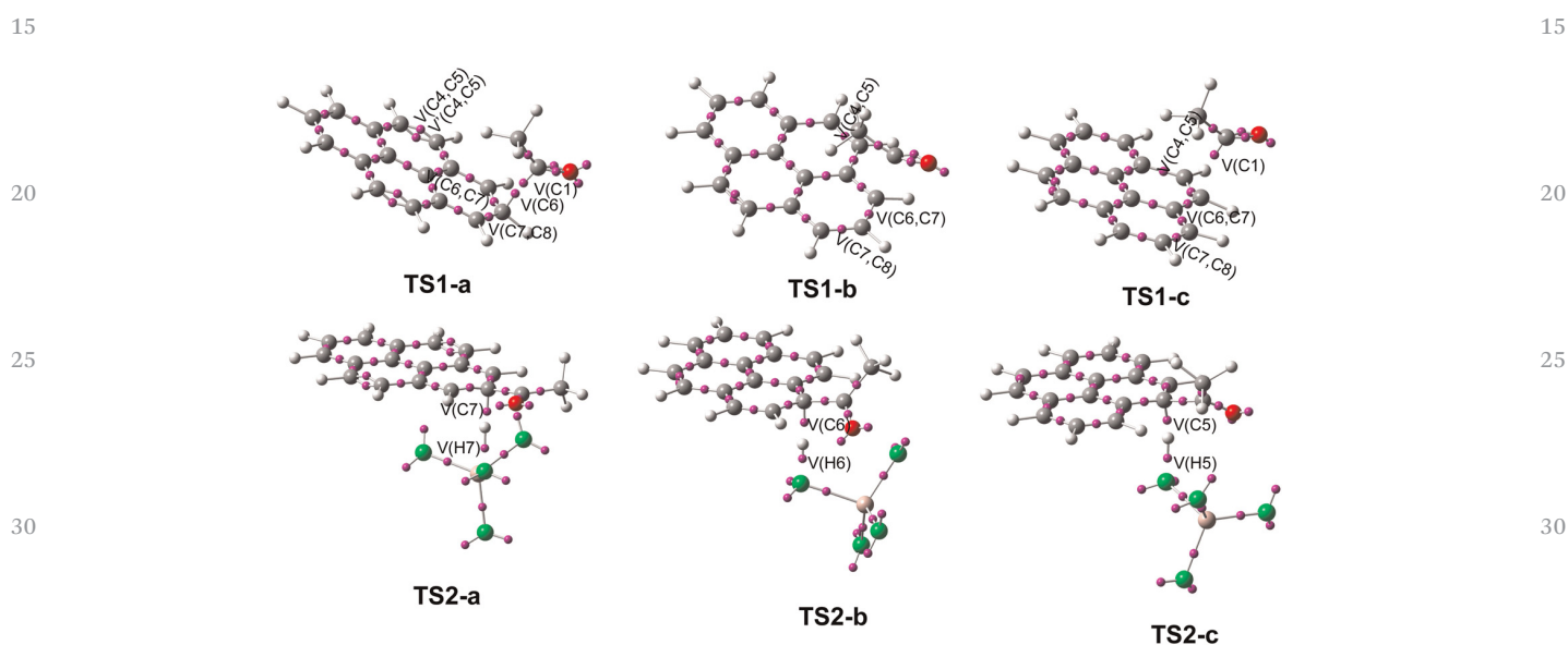
Fig. 10 ELF attractor positions of transition states TS1-a , TS1-b , TS1-c , TS2-a , TS2-b and TS2-c .
