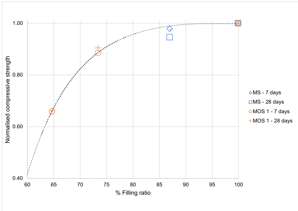
Figure 10: Normalised compressive strength evolution for the MS and MOS1 formulations at different curing times as a function of the filling ratio (the compressive strength is normalised by its value at a 100% filling ratio).
