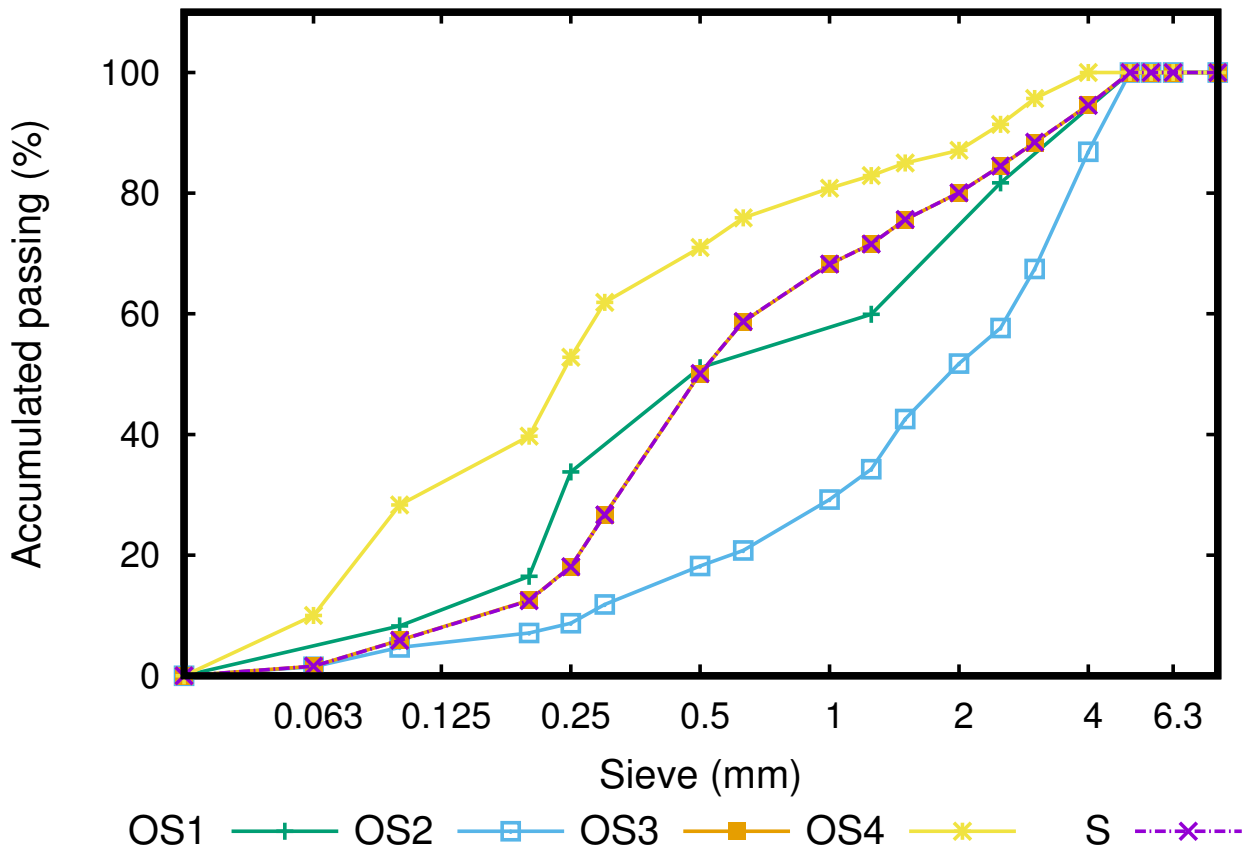
Figure 6: Particle size distribution of the different granular arrangements: classical sand S, optimised OS1, coarse OS2, sand-mimicking OS3, and fine OS4.
