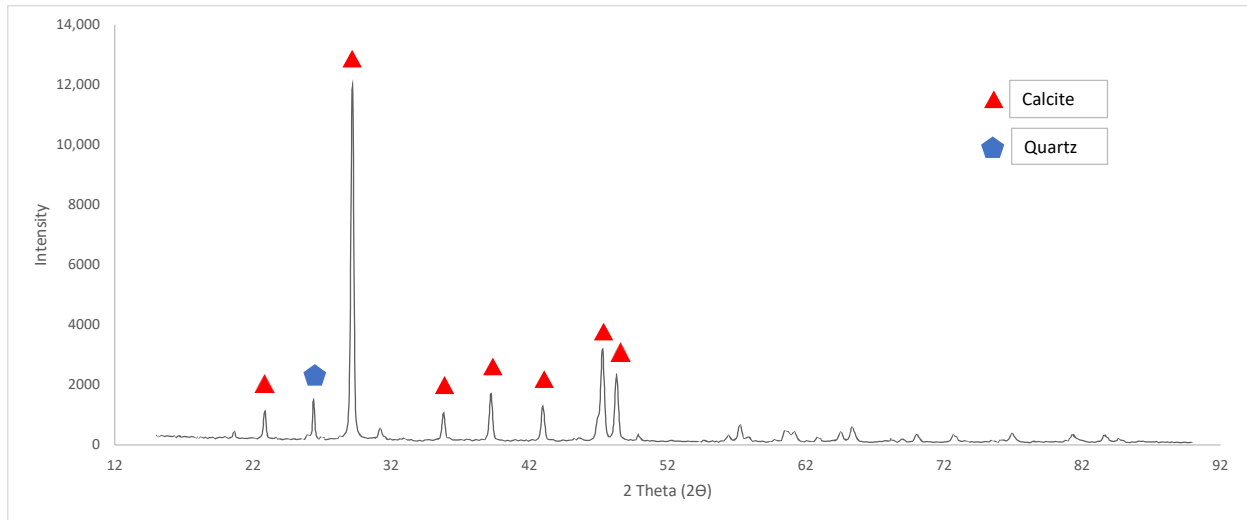
Figure 3: X-ray diffraction pattern of the Crassostrea gigas oyster shell.
