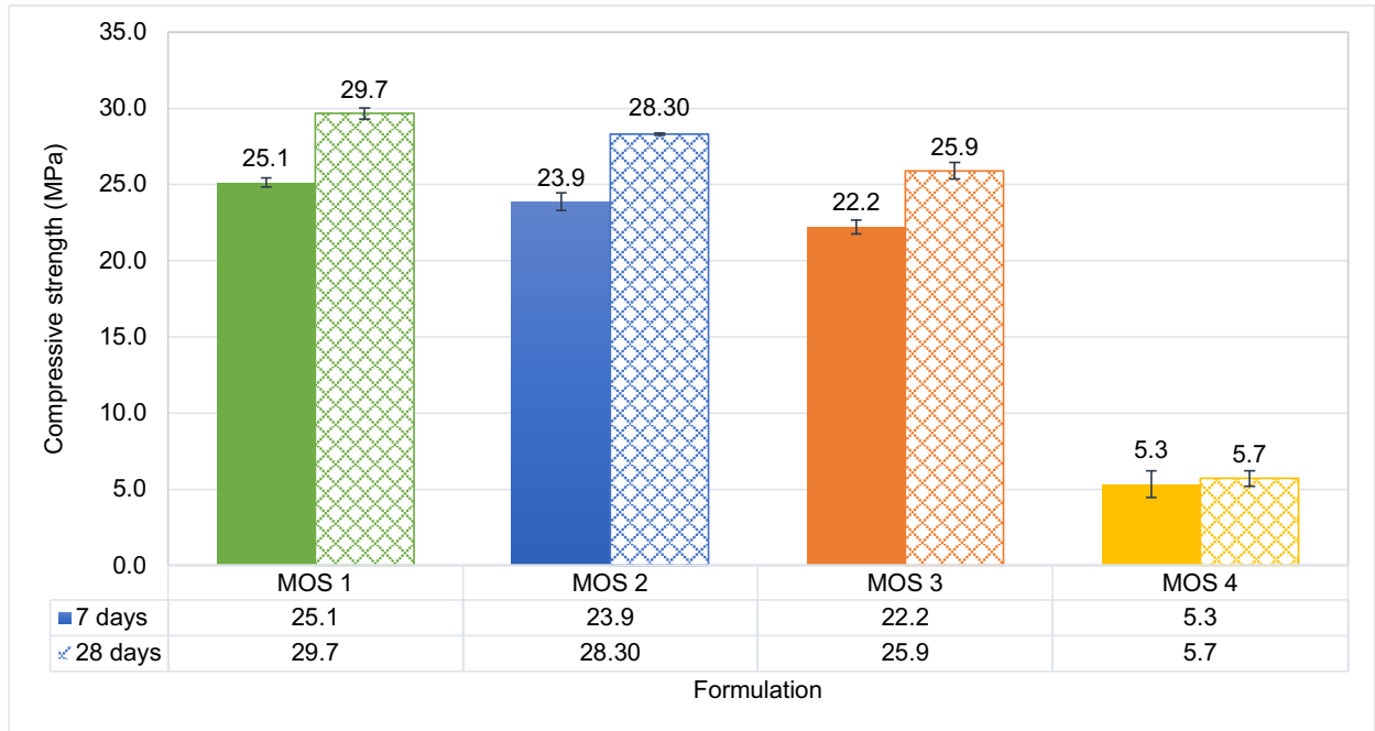
Figure 8: Compressive strength comparison of the oyster shell mortar formulations after 7 days (plain) and 28 days (cross-hatch) of curing at constant cement paste content. MS compressive strength: 45.4 \pm 0.6 MPa at 7 days, 59 \pm 2 MPa at 28 days.
