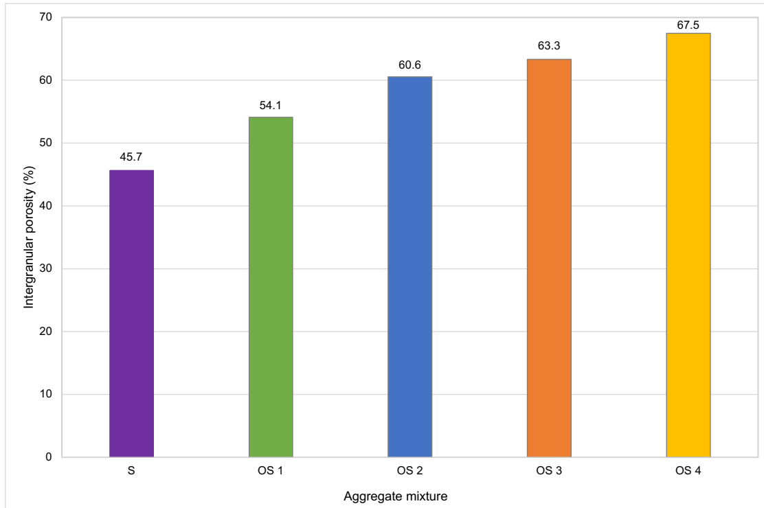
Figure 7: Intergranular porosity of the different granular arrangements: classical sand S (45.7%), optimised OS1 (54.1%), coarse OS2 (60.6%), sand-mimicking OS3 (63.3%), and fine OS4 (67.5%).
