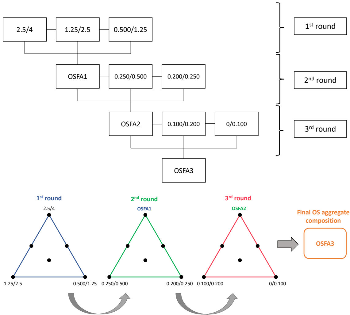
Figure 4: Principle of the optimisation of the oyster shell granular skeleton based on seven particle classes (2.5/4 mm, 1.25/2.5 mm, 0.500/1.25 mm, 0.250/0.500 mm, 0.200/0.250 mm, 0.100/0.200 mm, and 0/0.100 mm). OSFA1, OSFA2, and OSFA3, respectively, denote the resulting mixes after rounds #1, #2, and #3 of optimisation.
