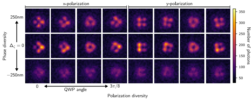
FIG. 2. PZ-stack for an unpolarized emitter shaped with an SEO element and modeled with PYPSPSTACK. Only the PSFs at the initial, middle, and final values of the defocus parameter \Delta\zeta used for the phase diversity in the retrieval of the BDPP shown in Fig. 3 are shown. For each \Delta\zeta , we show the PSFs for all polarization projections of diversity. This polarization diversity is generated by a rotating quarter wave plate followed by a projection onto linear horizontal or vertical polarization states.
