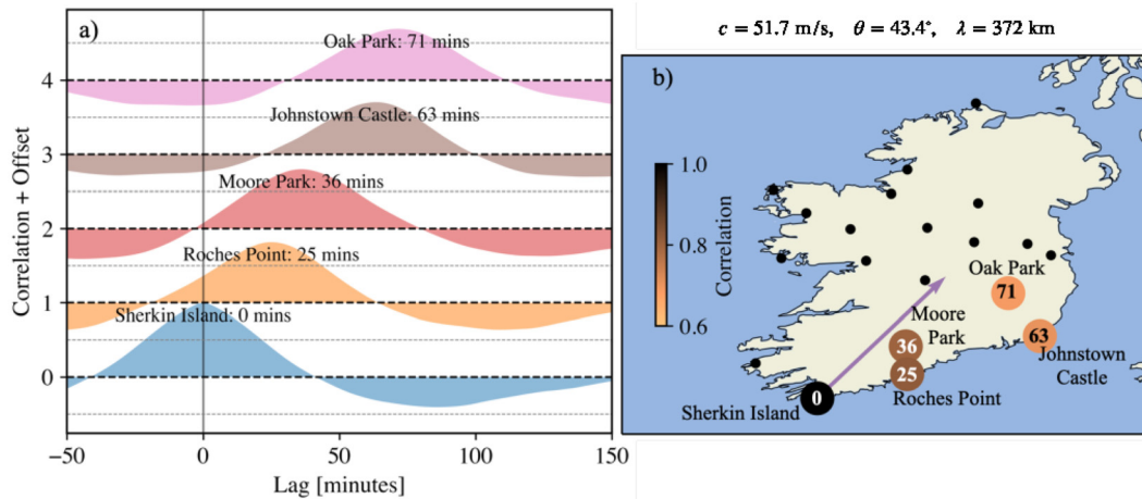
FIG. 6. (a) Cross-correlation between surface pressure data recorded by the Irish weather station network. (b) Map of the stations. The color scale represents the maximum correlation with respect to the Sherkin Island station, and the circled numbers indicate the associated time lag in minutes. The arrow indicates the estimated direction of the pressure disturbance traveling along the southern Irish coast, based on the cross-correlation analysis. Only correlations above 0.6 were considered.
