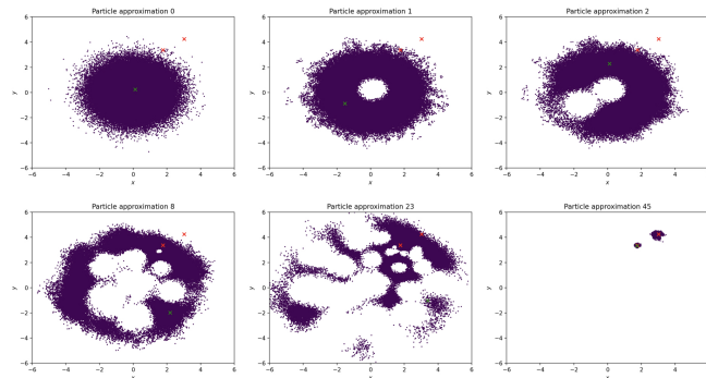
Figure 2 – Evolution of particles over some steps k . Particles are initially sampled from the prior p(\theta) and progressively evolve to particles located around the initially unknown source positions indicated by red crosses. Green crosses indicate the optimal measurement locations \xi_k^* obtained at each step k .
