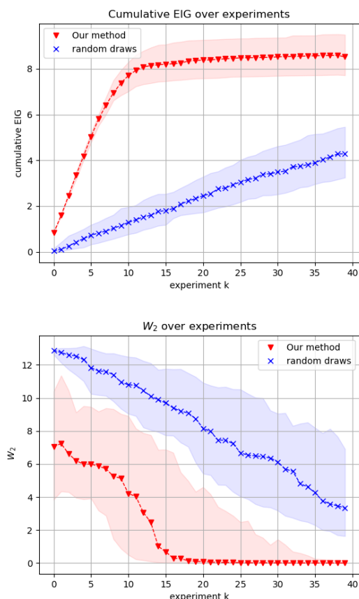
Figure 1 – Cumulative EIG adding each I_{PCE}^k (top) and L_2 Wasserstein distance between weighted particles at each step k and the true source locations (bottom) for our method (red) and random draws (blue). Lines and shaded regions represent the median, 25% and 75% quantiles over 150 rollouts.
