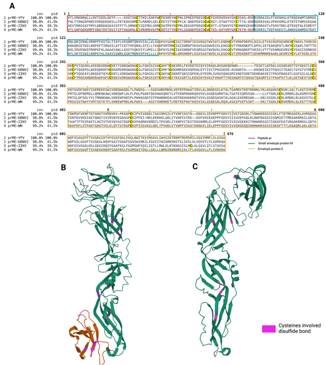
Figure 4. Disulfide bonds in flavivirus prM/E protein. (A) Alignment of prM/E protein sequence from YFV (POLG_YEFVA), DENV2 (POLG_DEN2N), WN (POLG_WNV9) and ZIKV (ARB08102.1). The cysteine positions are highlighted in yellow. (B) Crystallography structure of DENV2 prM/E (3C6E), with cysteine positions involved in disulfide bonds formation highlighted in pink. (C) Crystallography structure of ZIKV-E (5JHM), with cysteine positions involved in disulfide bonds formation highlighted in pink.
