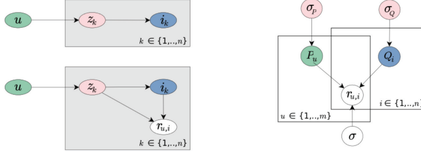
Figure 2 Dimensionality Reduction: Probabilistic Models (Mnih and Salakhutdinov, 2008; Ekstrand et al., 2011). (Left) Probabilistic Latent Semantic Analysis (PLSA). (Right) Probabilistic Matrix Factorization (PMF).
