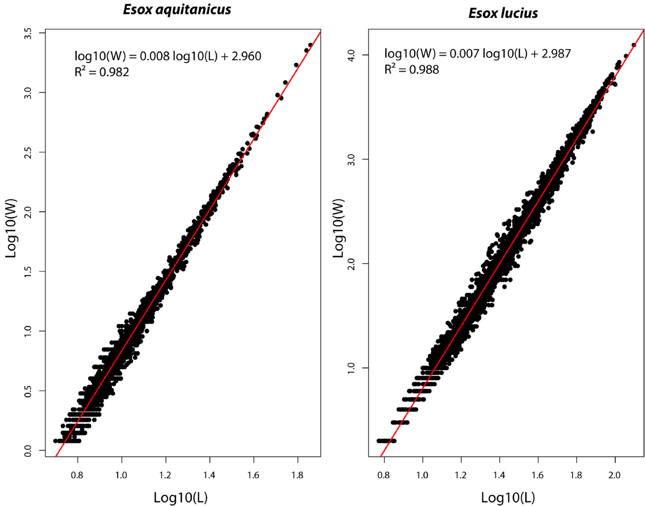
Fig. 5. Lengths ( L )–weights ( W ) regressions of Esox aquitanicus and Esox lucius . Data were log 10 transformed.
