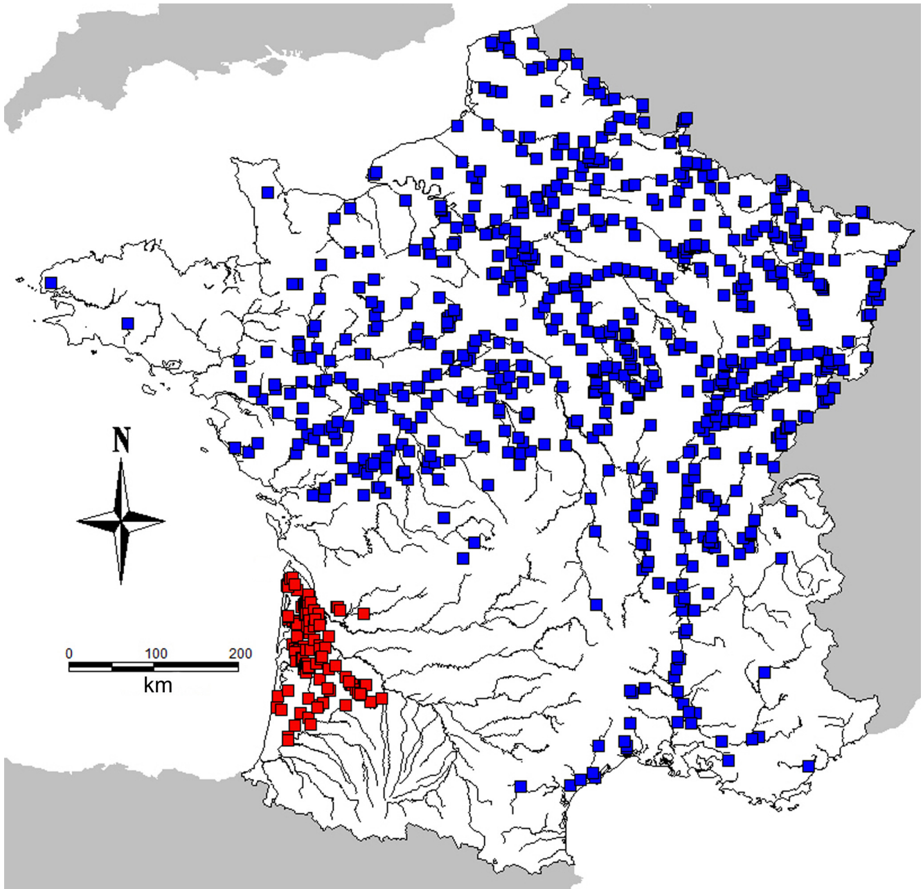
Fig. 4. Locations of both pike species ( Esox aquitanicus in red and Esox lucius in blue) from where lengths and weights data came.
