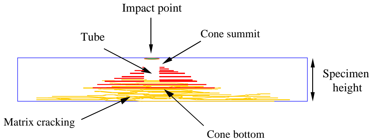
Fig. 7: Schematic visualization of damage in material thickness
