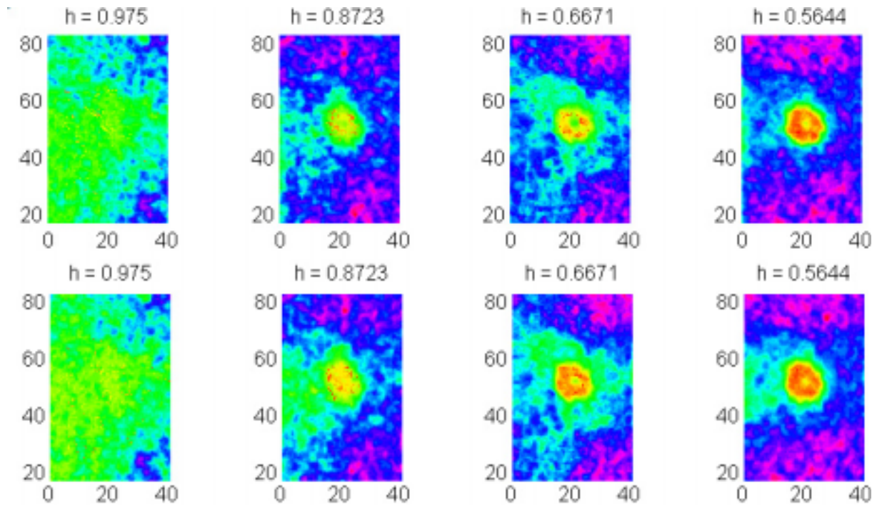
Fig. 8: Damage variation after post-impact fatigue. Above: Unifilo ® Glass E / Polyester impacted at 15J. At the bottom: Unifilo ® Glass E / Polyester impacted at 15J and fatigue during 20000 cycles at 31% of the tensile failure.
