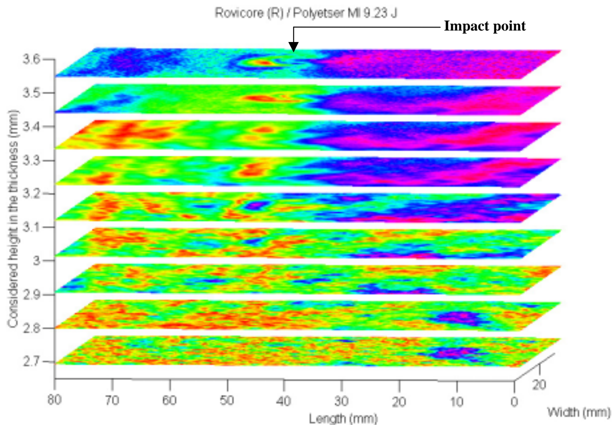
Fig. 9: Rovicore® / Polyester impacted at 9.32 J: visualisation near the impacted surface.
