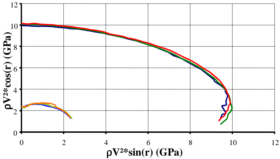
Fig. 4: Comparison of surfaces of rigidities for three Rovicore ® / Polyester samples
