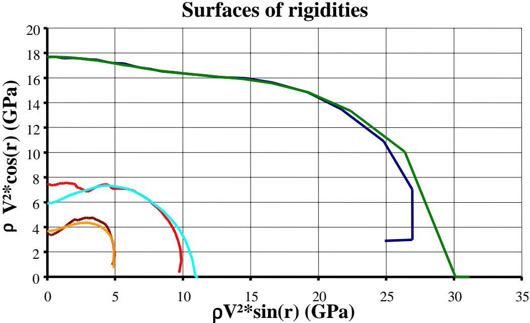
Fig. 6: Comparison of experimental and computed surfaces of rigidities for a Glass E / Phenolic unidirectional composite transversally woven with Glass E (10%)
