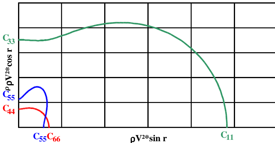
Fig. 2: Schematic surfaces of rigidities in the plane (1,3) for an orthotropic composite
