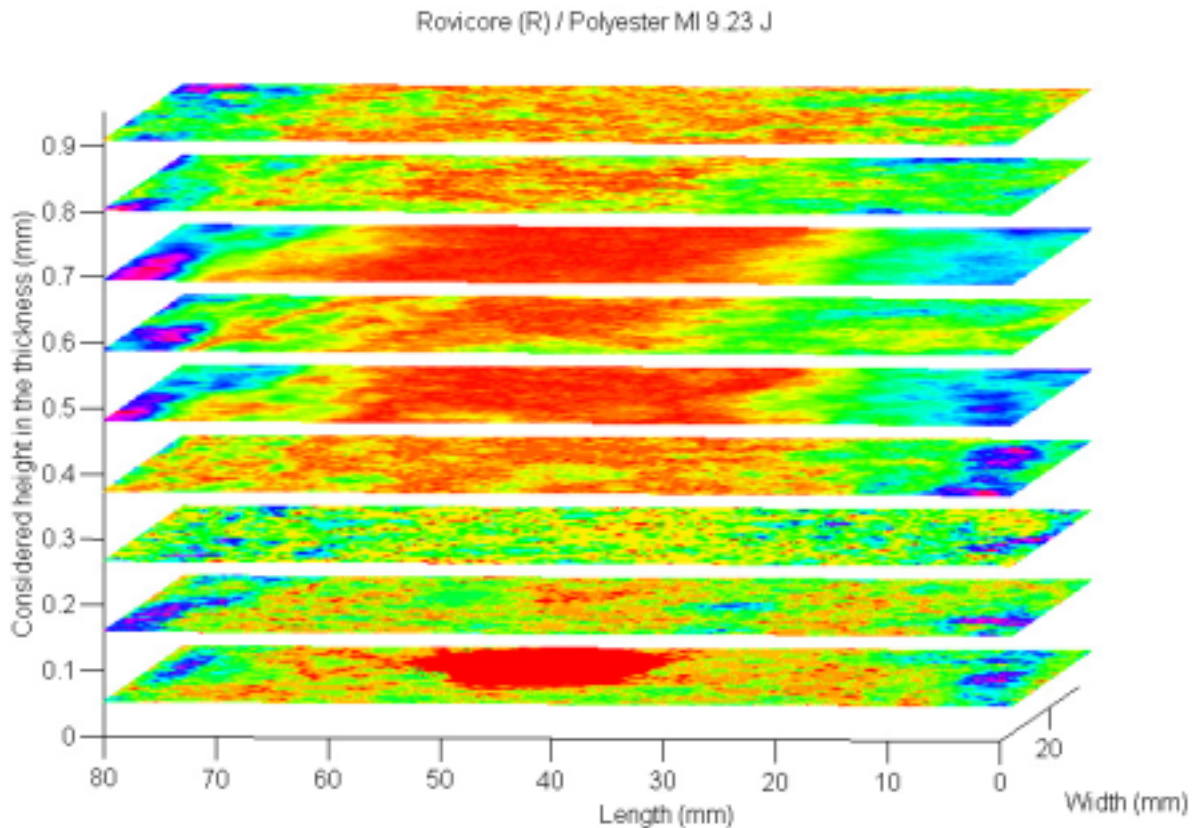
Fig. 10: Rovicore® / Polyester impacted at 9.32 J: visualisation near the non-impacted face.
