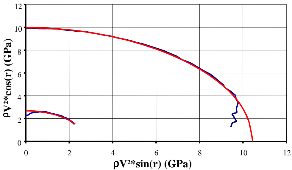
Fig. 5: Comparison of experimental and computed surfaces of rigidities for a Rovicore ® / Polyester composite
