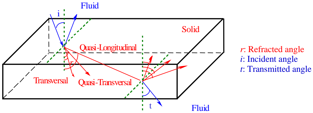
Fig. 1: Ultrasonic waves in a solid induced by an incident plane wave
