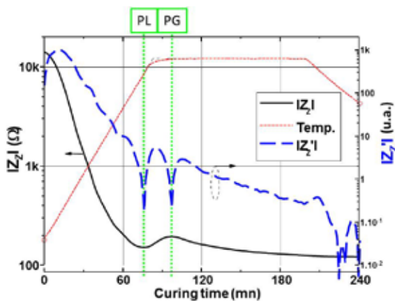
Fig. 1 Changes in |Z_L| and its first time derivative |Z'_L| (arbitrary units) during oven-curing of an [0^\circ_8] sample. PL=minimum viscosity point, PG=gel point.
