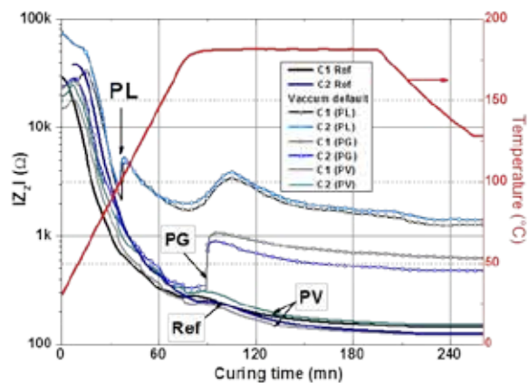
Fig. 2 Vacuum default effect on the through-the-thickness impedance |Z_z| ( f = 10 kHz) during oven curing of [0^\circ_8] laminates.
