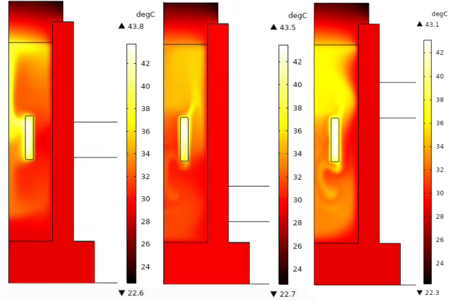
(a) B_z = 0.2 T and (b) B_r = -0.2 T (c) B_r = 0.2 T and coil.
