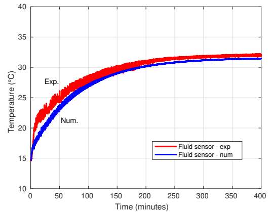
Fig. 6: Experimental/numerical cross-validation with the presence of the magnet, Z = 6.5\text{ cm} .
