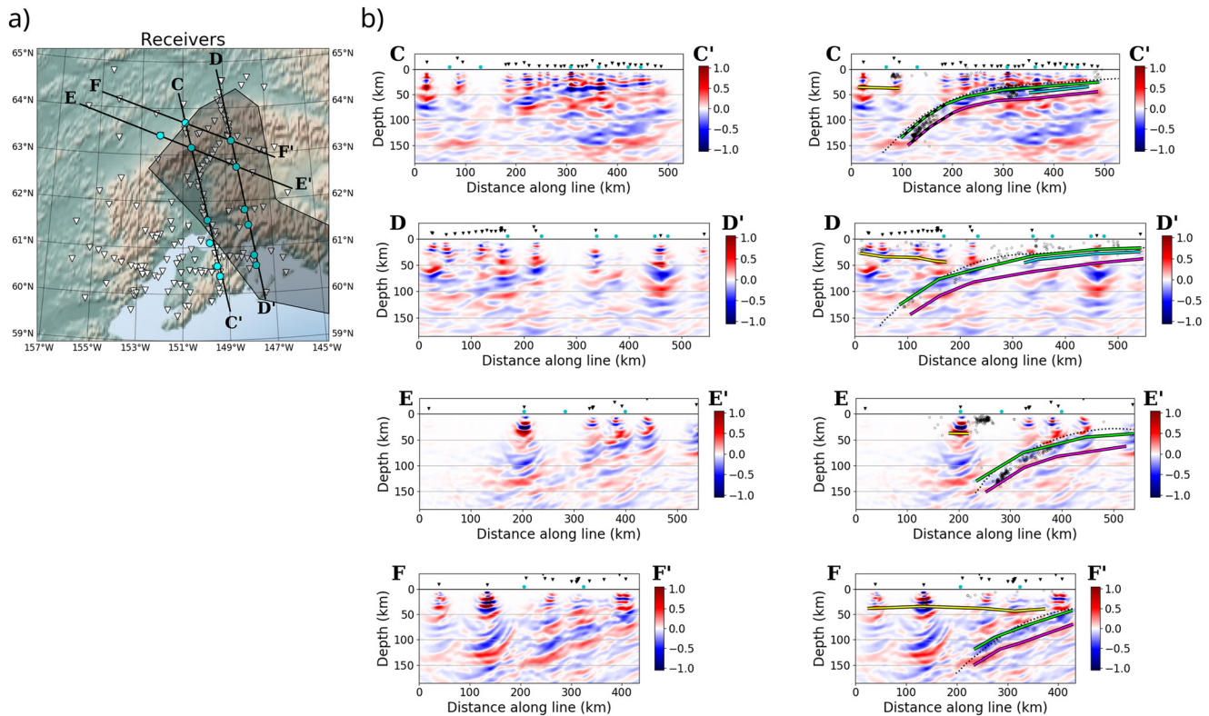
Figure 5. (a) Location of cross-sections through the thickened Yakutat subducting slab. (b) Raw and interpreted cross sections. Green is the slab top, magenta is the Yakutat Moho, cyan is the subduction channel inferred by Kim et al. (2014) and yellow is the continental Moho. See Figure 4 caption for other details.
