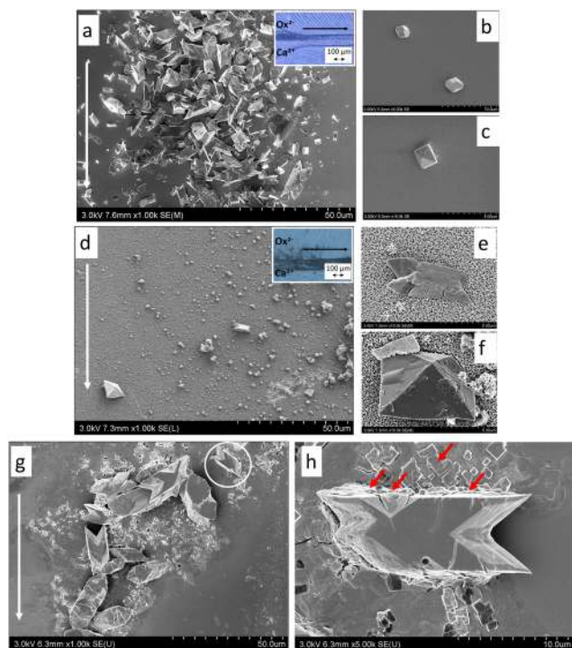
Fig. 3 Crystallization of CaOx in the microchannel after infusion of calcium and oxalate solutions. a–c Scenario A (SA): uncoated channel – a) SEM-FEG image of the glass coverslip at 300 \mu\text{m} from the microchannel junction with an optical micrograph of the microchannel in the insert. b and c) SEM images of crystals collected at the end of the channel. d–f) Scenario B (SB): CHA coated channel – d) SEM-FEG image of the glass coverslip at 300 \mu\text{m} from the microchannel junction with an optical micrograph of the microchannel in the insert and enlarged images of crystals formed in the channel. g) Scenario C (SC): SEM-FEG image of the CHA coated coverslip at 300 \mu\text{m} from the microchannel junction. The white arrow in all figures indicates the direction of the flow. h) Magnification of the zone delimited by a white circle in image g). The red arrows indicate similar protuberance structures on the surface of CHA and CaOx crystals. The same images are provided at higher format in the ESI.†
