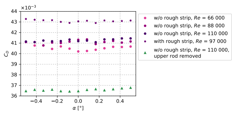
Figure 10: Cylinder in rotation: drag coefficient of a slightly inclined cylinder in axial flow, experimental results.
