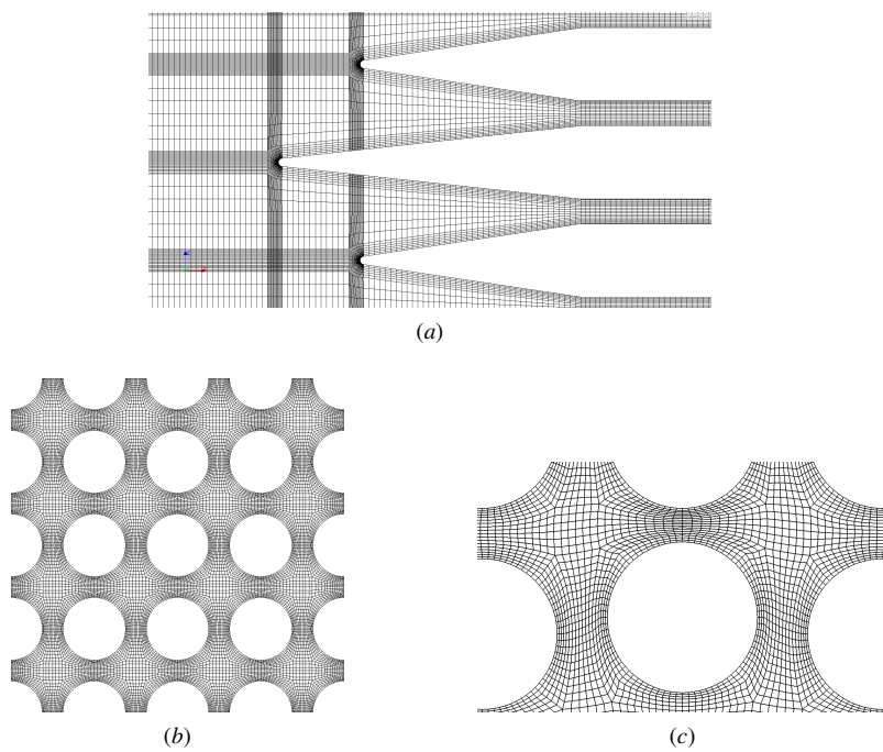
Figure 5: Section views of the mesh: (a) side view at y = 0 , (b) front view for x/D_h \in [0; 39] , and (c) detailed front view in a translation case ( Z = 5 mm).
