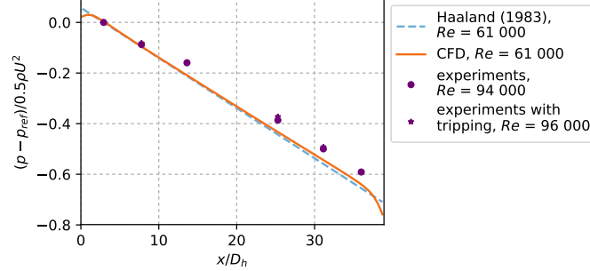
Figure 9: Non-dimensional pressure losses along the model. CFD values are taken from a line parallel to the x -axis at the centre of a wide channel ( y/P = z/P = 0.5 ). Each experimental point is obtained by averaging the values of the 16 pressure taps at the corresponding section. The reference pressure is chosen to be the one at the first section ( x/D_h = 2.9 ).
