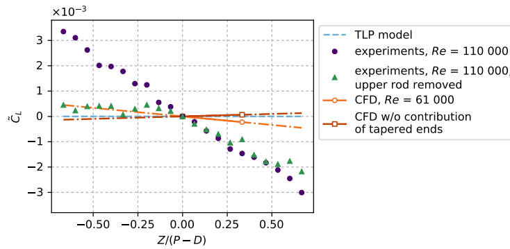
Figure 16: Cylinder in translation: comparison of lift coefficients obtained in the experiments, the numerical simulations and the TLP model (see discussion in § 4).
