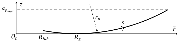
Fig. 1. Profile definition of the high-feed milling tool
