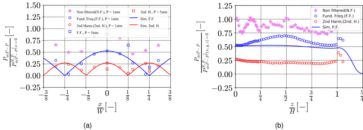
Figure 2. Spatial acoustic pressure characterization along acoustic axis : (a) along Ox and (b) along Oz .
