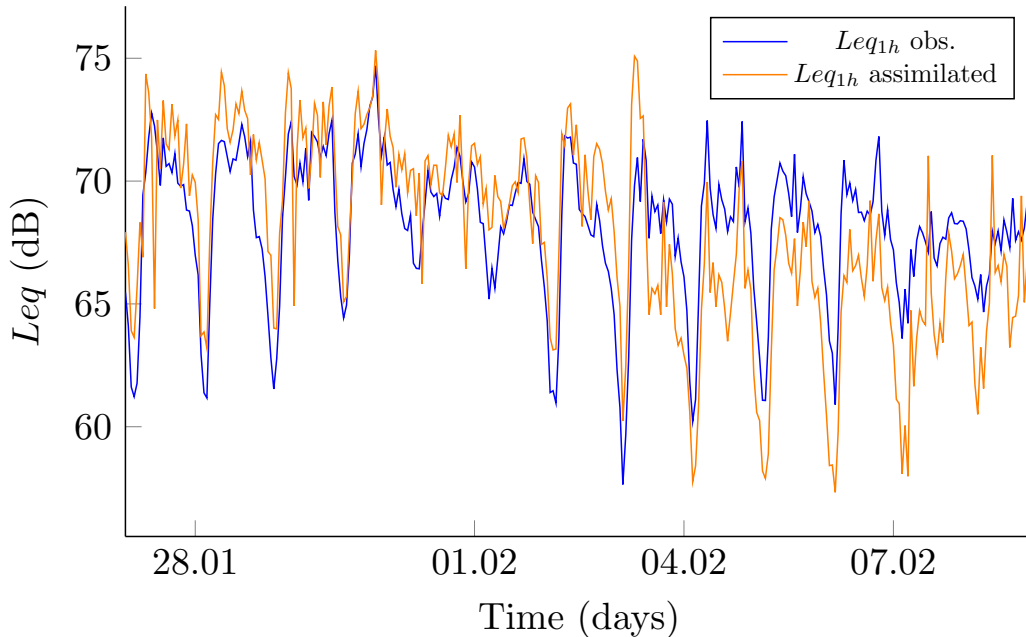
Figure 9: time evolution of the observed LA_{eq,1h} and the leave-one-out data assimilation process output for the sensor point colored in black in figure 3
