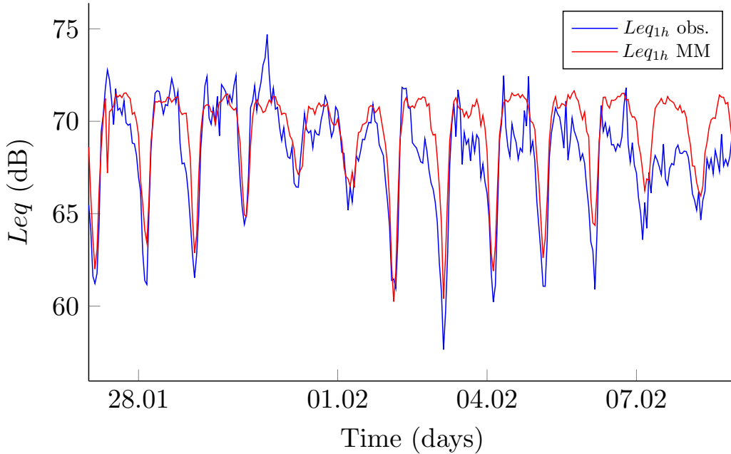
Figure 4: time evolution of the observed LA_{eq,1h} and the meta-model output for the sensor point colored in black in figure 3
