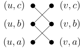
Figure 5: The tensor product of a K_2 graph uv and the P_3 graph abc . Here, the set of degree 1 vertices is an MEG-set.
