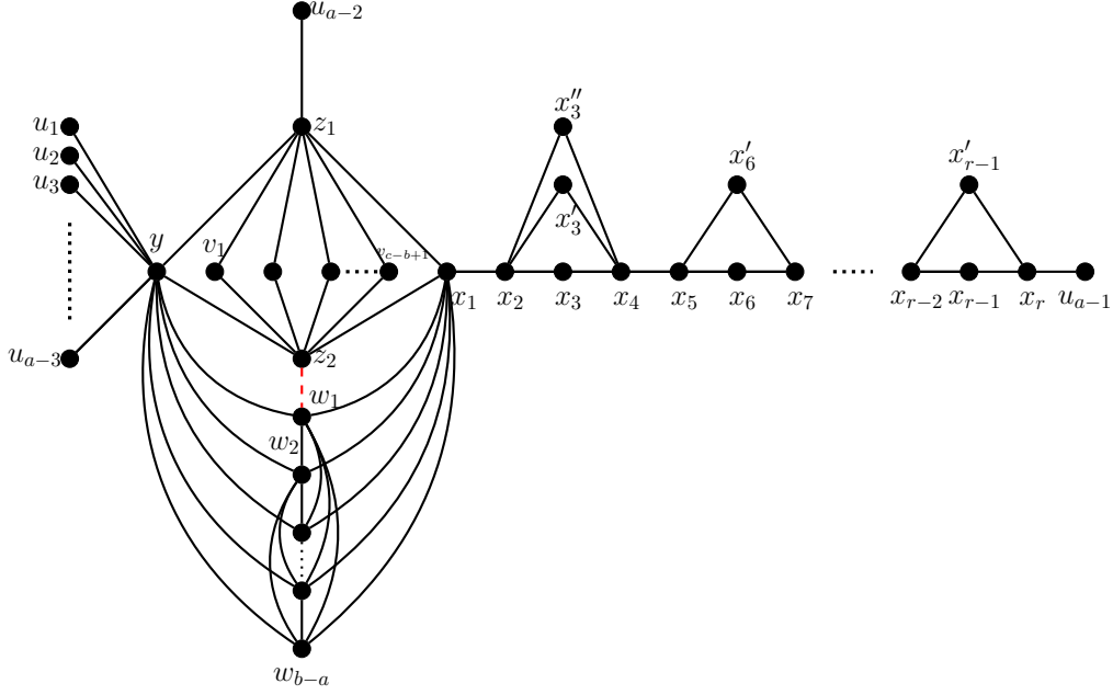
Figure 3: The structure of G_{a,b,c,d} . The red dashed edge between z_2 and w_1 represents an edge/non-edge depending on the values of a and b .
