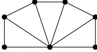
Figure 4: A 2-connected interval graph with a non-extremal MEG-set. Note that the set of all vertices except the universal vertex is an MEG-set.
