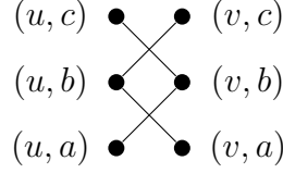
Figure 5: The tensor product of a K_2 graph uv and the P_3 graph abc . Here, the set of degree 1 vertices is a MEG-set.
