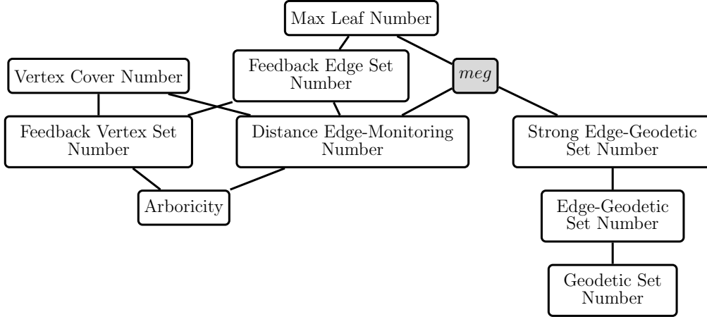
Figure 1: Relations between the parameter meg and other structural parameters in graphs (with no isolated vertices). For the relationships of distance edge-monitoring sets, see [16]. Edges between parameters indicate that the value of the bottom parameter is upper-bounded by a function of the top parameter. Figure reproduced from [14].
