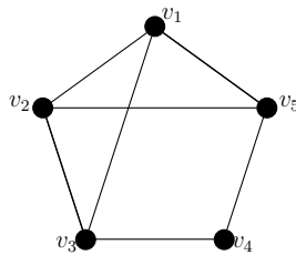
Figure 2: A graph G with 2 = g(G) < 3 = eg(G) < 4 = seg(G) < 5 = meg(G) . Note that, a minimum geodetic set of G is \{v_3, v_5\} , a minimum edge-geodetic set of G is \{v_1, v_2, v_4\} , a minimum strong edge-geodetic set of G is \{v_1, v_2, v_3, v_4\} (the assigned shortest paths between a pair of adjacent vertices is the edge between them, and between a pair of non-adjacent vertices is the 2-path through v_5 ) and a minimum MEG-set of G is \{v_1, v_2, v_3, v_4, v_5\} .
