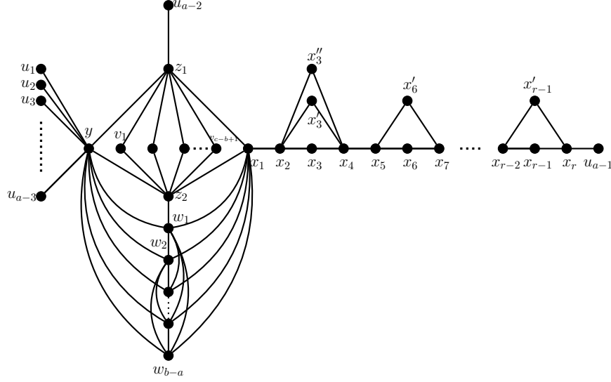
Figure 3: The structure of G_{a,b,c,d} .
