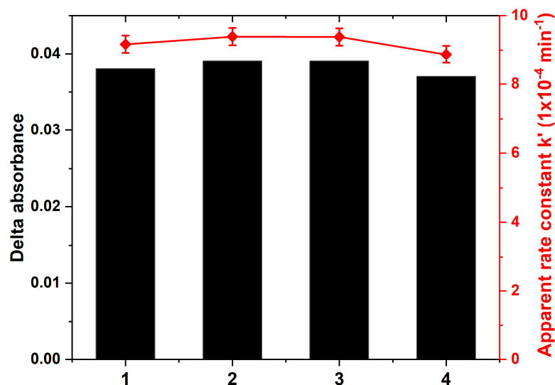
Figure 13. Photostability of the nanocomposite TiO 2 /SiO 2 -np film (sample B) of four cycles photocatalytic degradation.
