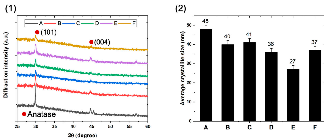
Figure 3. Structural properties of the nanocomposite \text{TiO}_2/\text{SiO}_2 -np film: (1) X-ray diffractograms with \theta-2\theta mode; (2) average crystallite size of the \text{TiO}_2 matrix.
