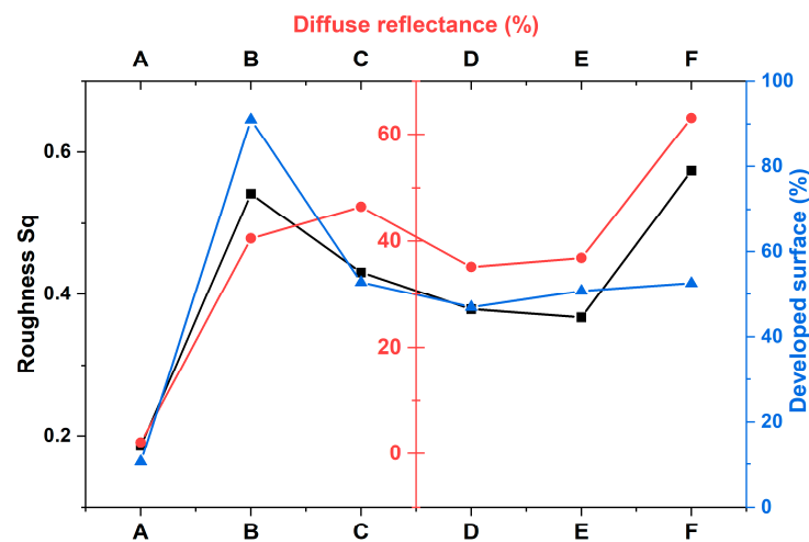
Figure 10. Correlation between the diffuse reflectance (at 410 nm) with the surface roughness S_q and the developed surface of the nanocomposites \text{TiO}_2/\text{SiO}_2 -np films.
