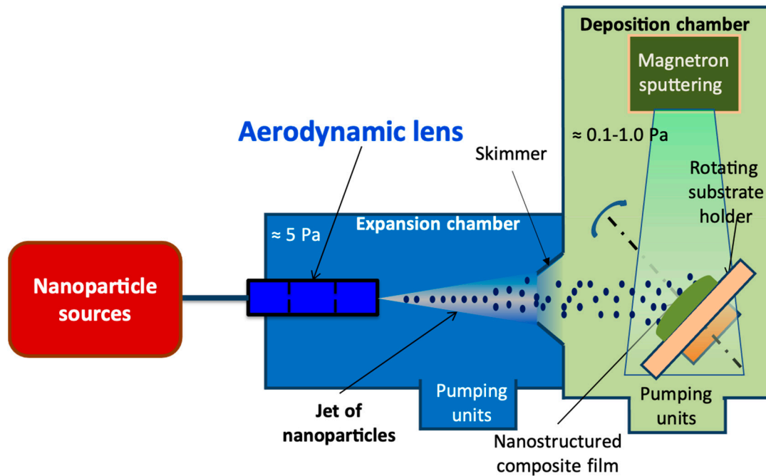
Figure 1. Drawing of the process for nanocomposite thin film synthesis allows independent control of nanoparticles and matrix deposition [31].
