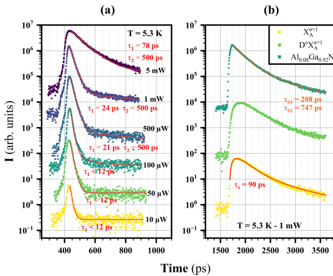
FIG. 11. (a) Time-resolved photoLuminescence (TRPL) results obtained on the complete heterostructure (GaN/ \text{Al}_{0.08}\text{Ga}_{0.92}\text{N} /GaN) for the decay of the free exciton X_A^{n=1} as a function of laser power. The red lines represent bi-exponential and mono-exponential fits of these decays. (b) TRPL results obtained on the etched heterostructure ( \text{Al}_{0.08}\text{Ga}_{0.92}\text{N} /GaN) for the three main transitions operating in the sample: X_A^{n=1} - D^0 X_A^{n=1} - \text{AlGaIn} . The decays are measured for the same laser power to study the dynamics of recombination mechanisms in the structure. The solid lines correspond to the decay fits performed with models consistent with the structure's dynamics. The baseline of each spectrum is shifted vertically for clarity.
