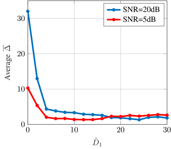
Fig. 17: Evolution of \bar{\Delta} with \tilde{D}_1 for \tilde{D}_2 = 30 for the Nokia dataset.
