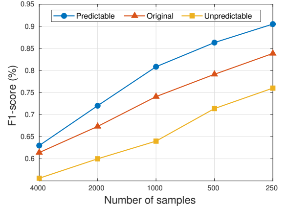
(b) Average f1-score, for several sample sizes M
