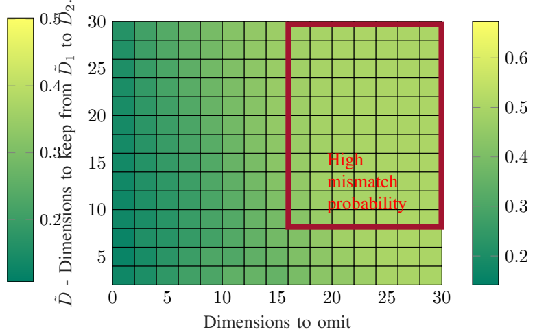
(b) Average MP
