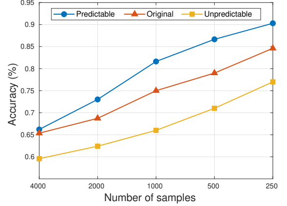
(a) Average accuracy, for several sample sizes M
