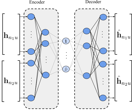
Fig. 4: A representative block diagram of AE2.
