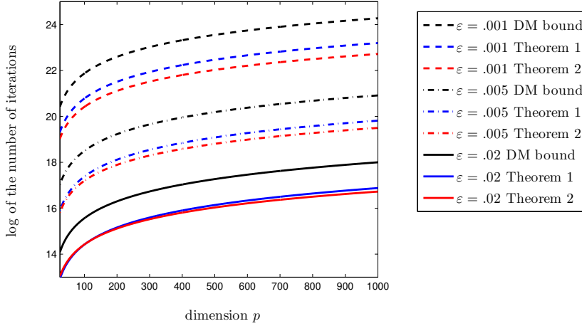
Figure 1: Plots showing the logarithm of the number of iterations as function of dimension p for several values of \epsilon . The plotted values are derived from (3)-(5) using the data m = 10 , M = 20 , W_2^2(\nu_0, \pi) = p + (p/m) .
