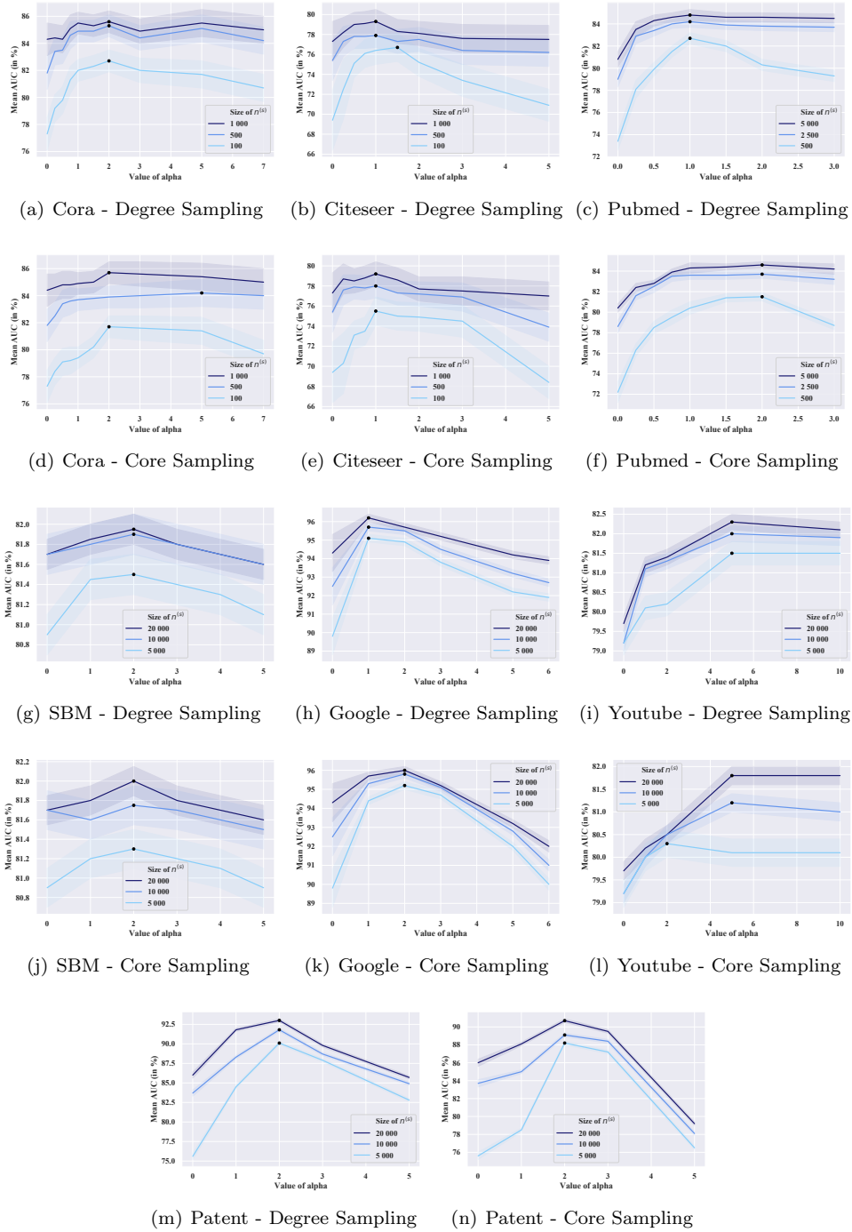
Figure C.6: Optimal values of hyperparameter \alpha for degree-based and core-based node sampling w.r.t. mean AUC scores on validation sets, for Variational FastGAE models and for all graphs.
