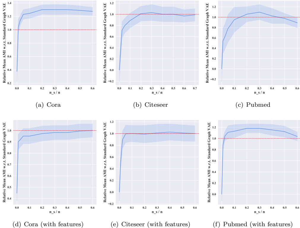
Figure 4: Summarized results for node clustering on the medium-size graphs Cora, Citeseer and Pubmed: relative mean AMI scores of degree-based Variational FastGAE models w.r.t. standard Graph VAE depending on the proportion of sampled nodes n_{(S)}/n in decoders. We observe that, even for relatively low n_{(S)}/n proportions, Variational FastGAE achieves comparable or even slightly better performances w.r.t. standard Graph VAE (results above the red line).
