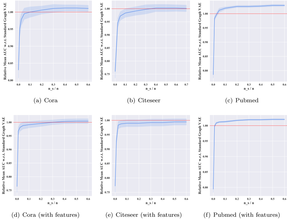
Figure 3: Summarized results for link prediction on the medium-size graphs Cora, Citeseer and Pubmed: relative mean AUC scores of degree-based Variational FastGAE models w.r.t. standard Graph VAE depending on the proportion of sampled nodes n_{(S)}/n in decoders. We observe that, even for relatively low n_{(S)}/n proportions, Variational FastGAE achieves comparable or even slightly better performances w.r.t. standard Graph VAE (results above the red line).
