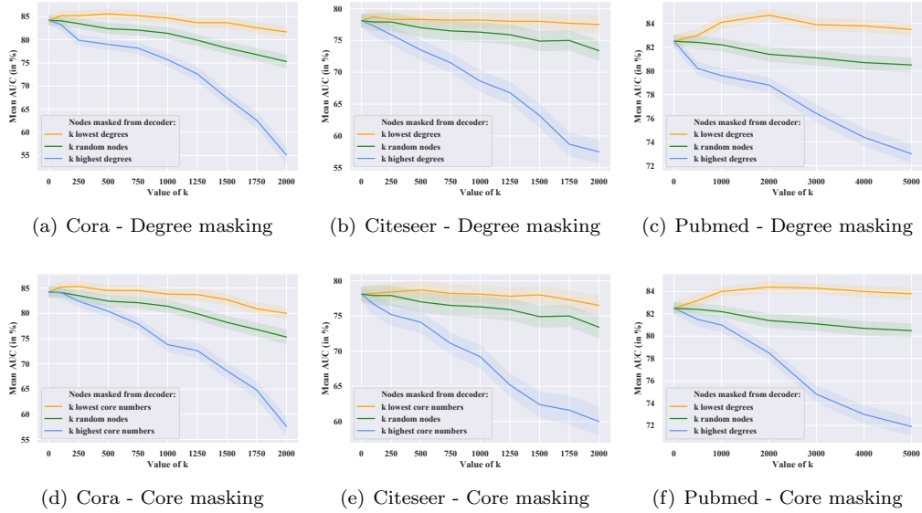
Figure 1: Link prediction on featureless Cora, Citeseer and Pubmed using standard Graph VAE models, but trained while masking k nodes and their connections from the decoder/reconstruction loss. AUC scores are averaged over 100 runs with random train/test splits.
