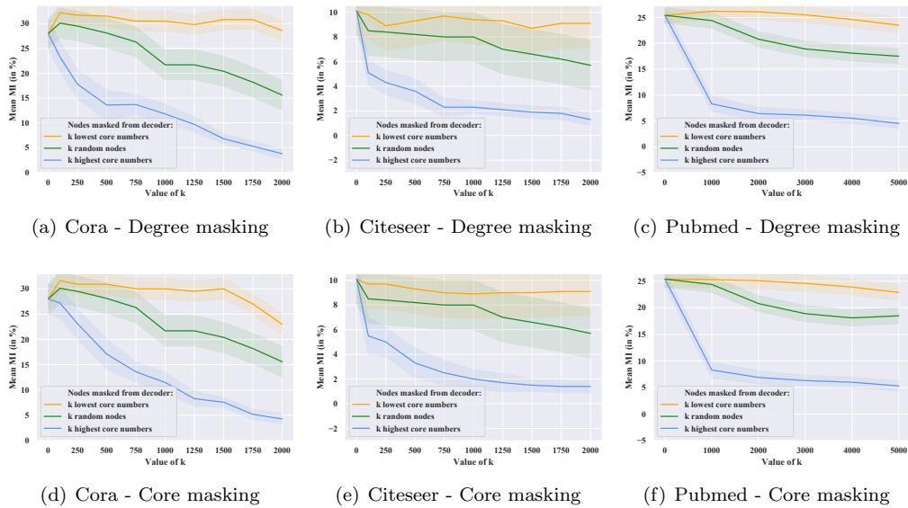
Figure 2: Node clustering on featureless Cora, Citeseer and Pubmed using standard Graph VAE models, but trained while masking k nodes and their connections from the decoder/reconstruction loss. Adjusted MI scores are averaged over 100 runs with random train/test splits.
