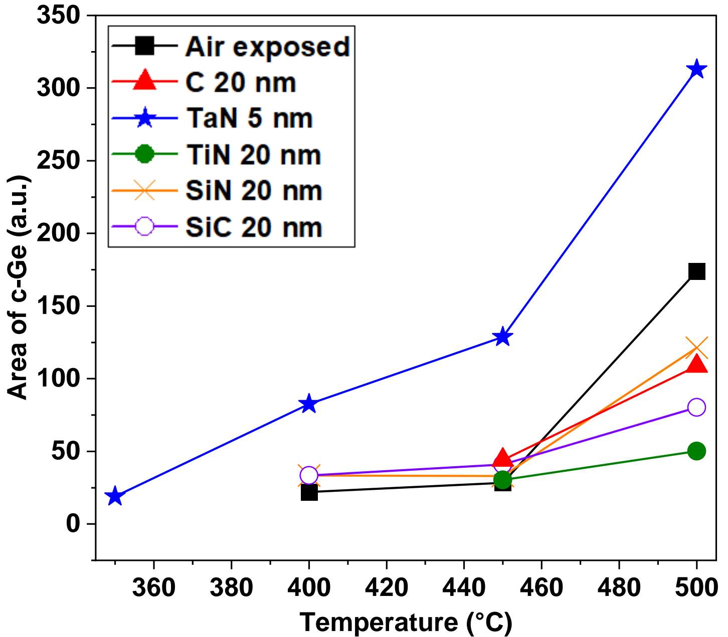
Figure 8: Evolution of c-Ge peak area obtained from Raman spectra at increasing annealing temperature.
